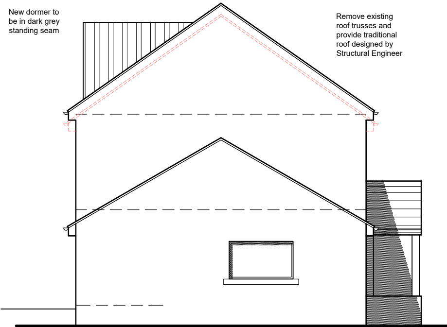
East Elevation
