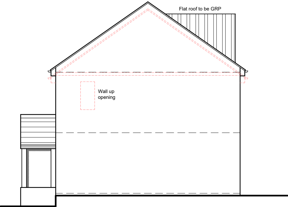
West Elevation
