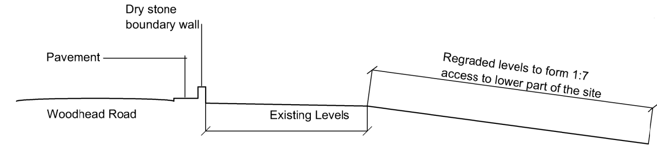
Typical Cross Section of proposed new access 1:200 scale
