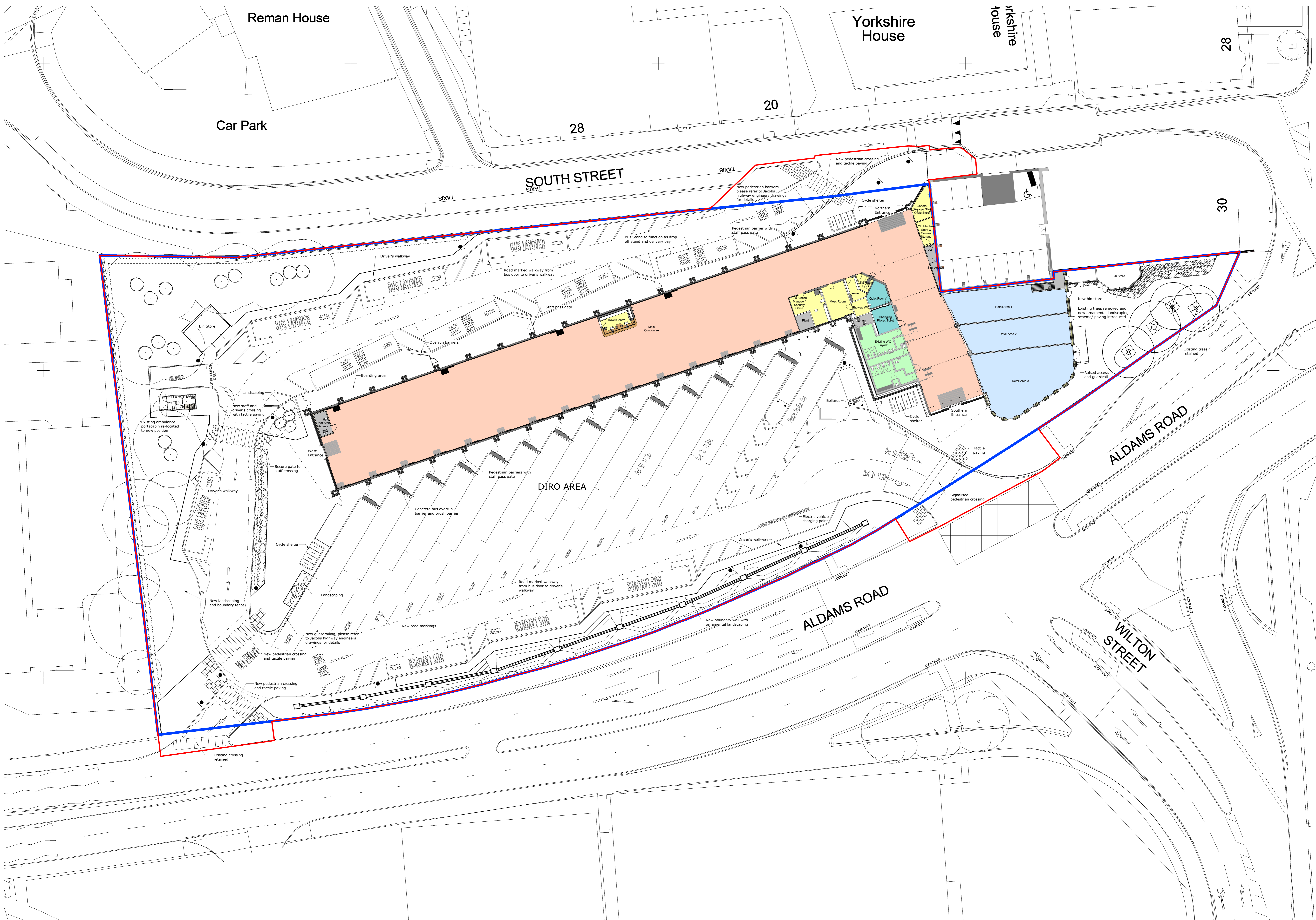
Proposed Site Plan SCALE: 1 : 200
