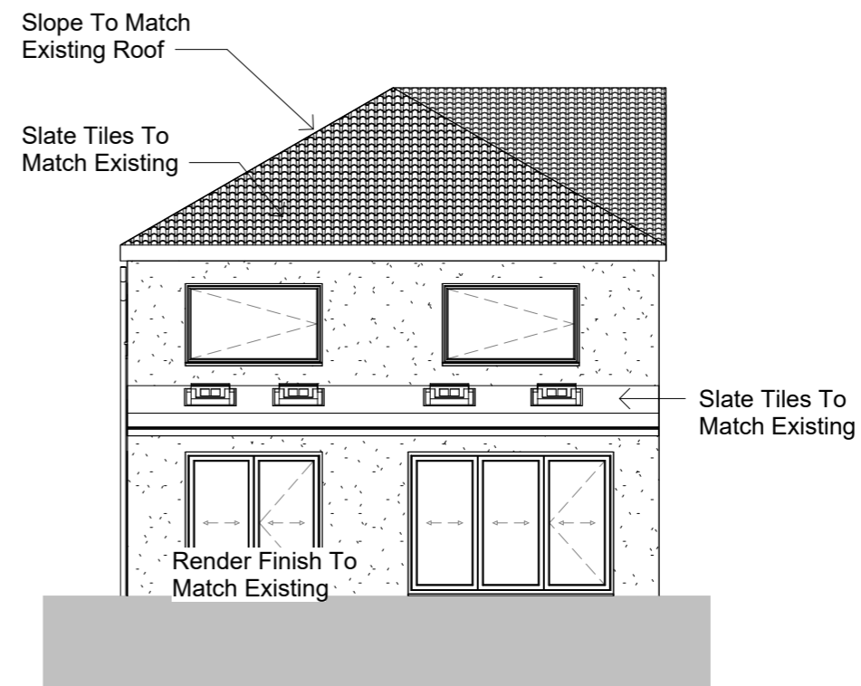
Proposed West North West (Rear)
