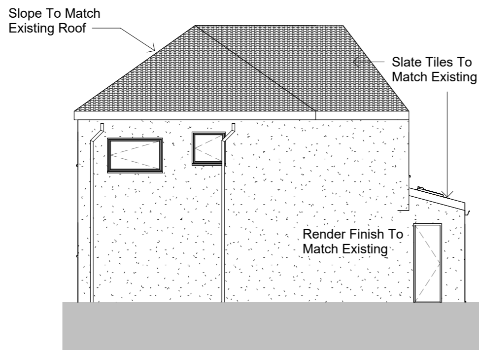
Proposed North East North (Right)
