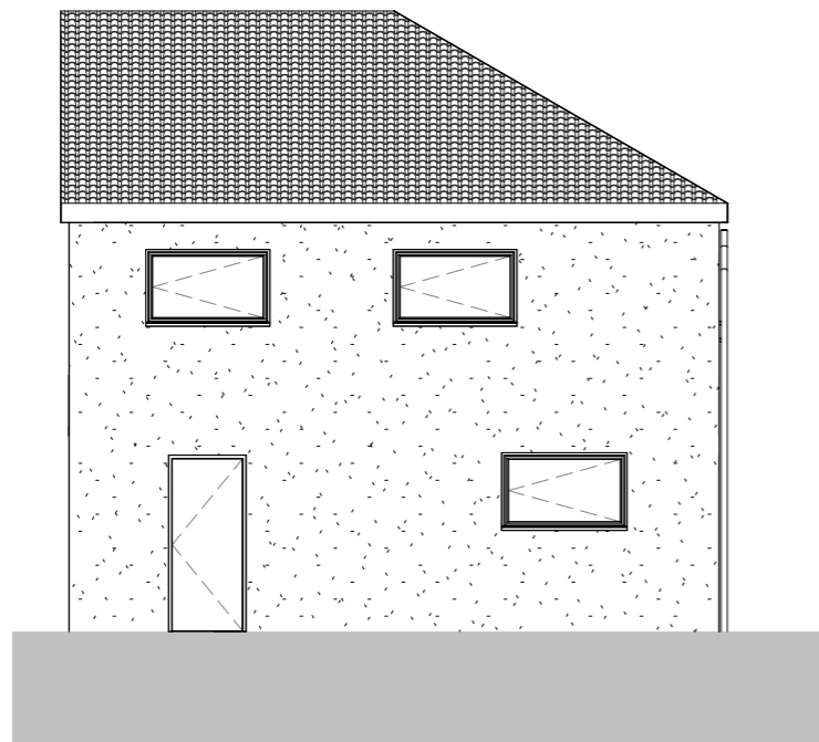
Proposed East South East (Front)
