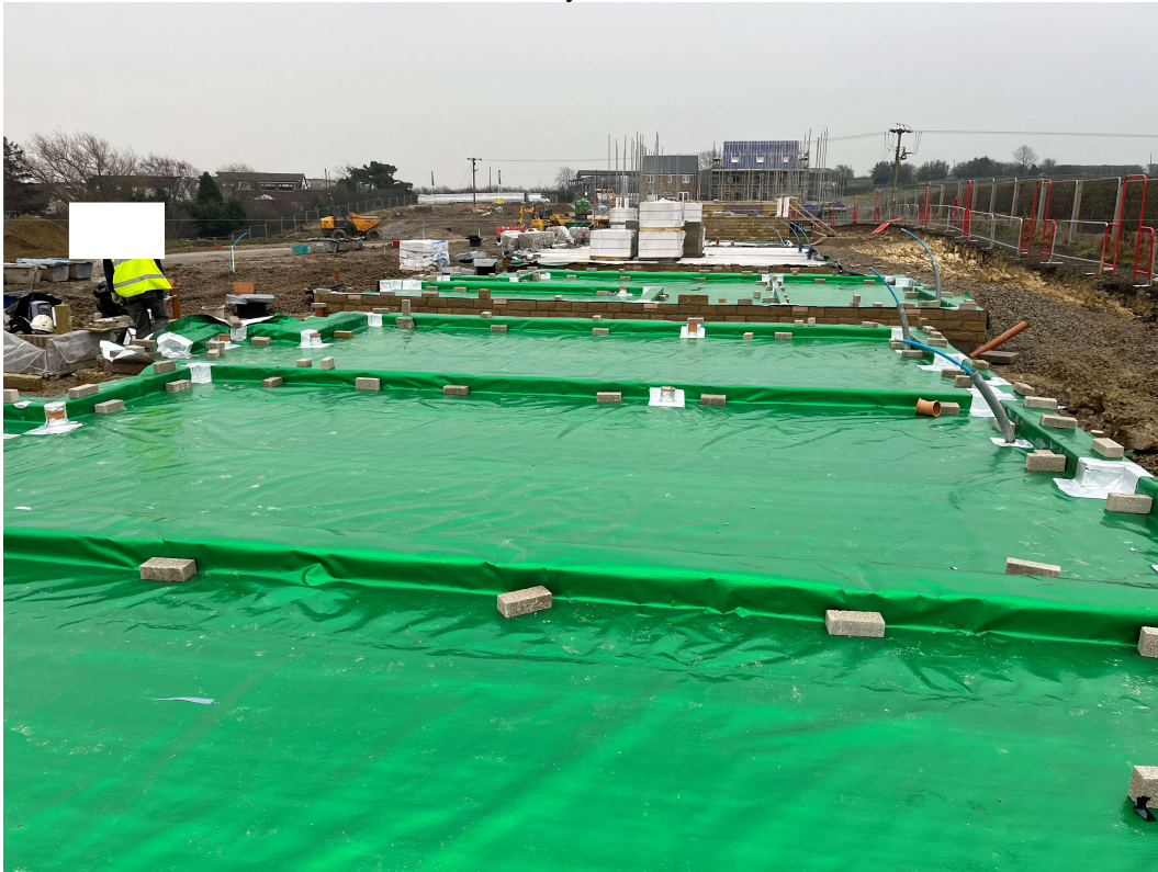
Plot 20 – Overall membrane layout
