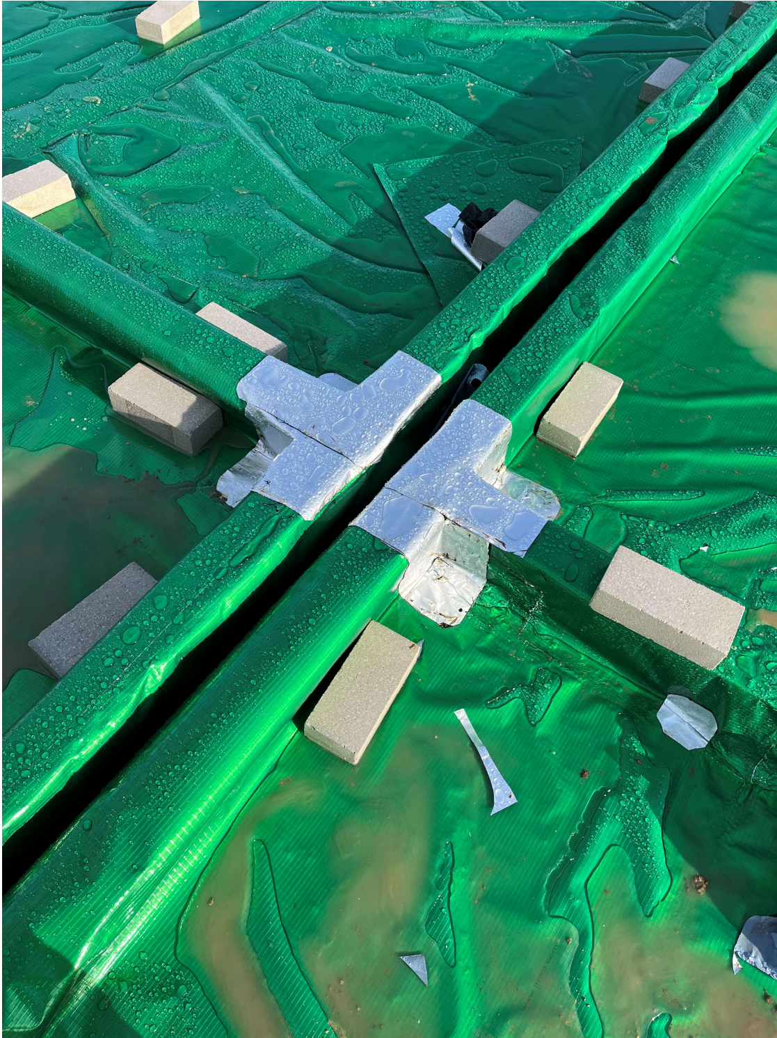
Plots 15 & 16 – Party wall membrane layout and jointing
