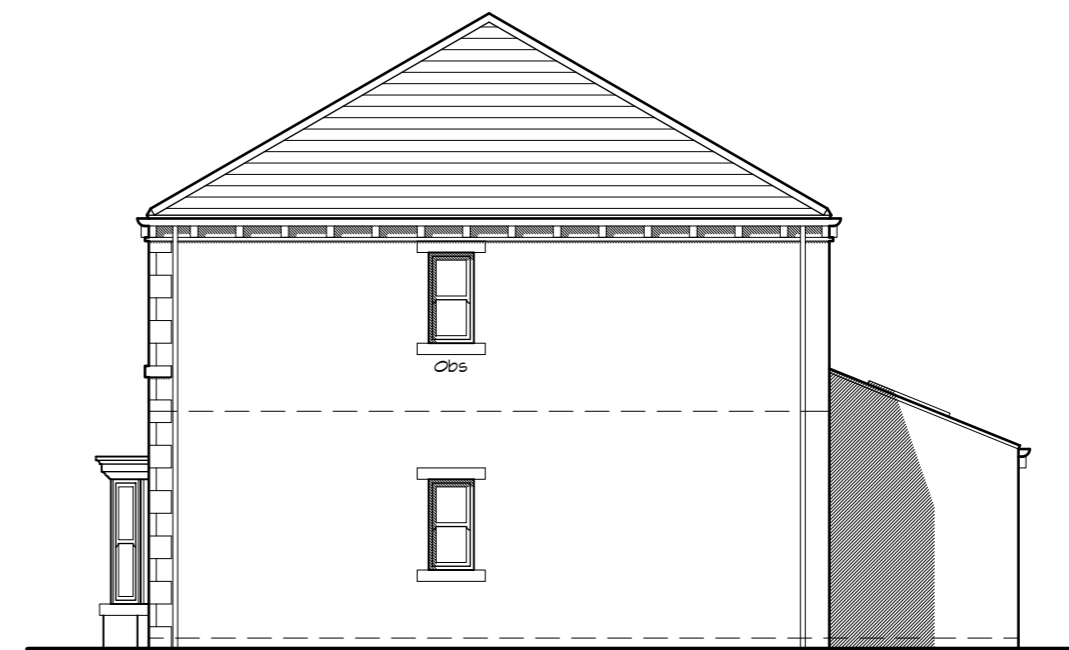
Side Elevation
