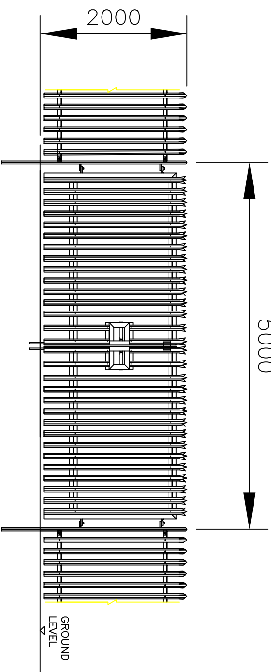
ELEVATION ON ENTRANCE GATE SCALE 1:50
