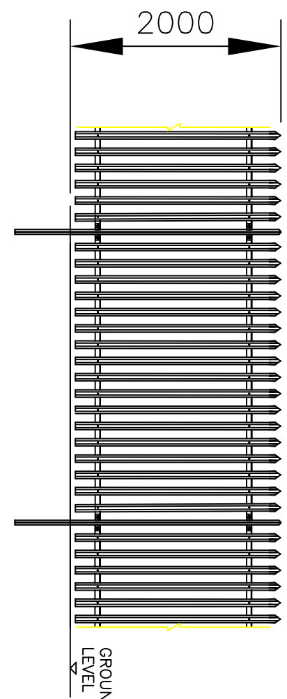
ELEVATION ON PAUSADE FENCING SCALE 1:50
