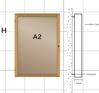
ITEM H. ONE X NEW POSTER CASE SIZE. 488mm x 663mm. H.A.G. 1.2m.
