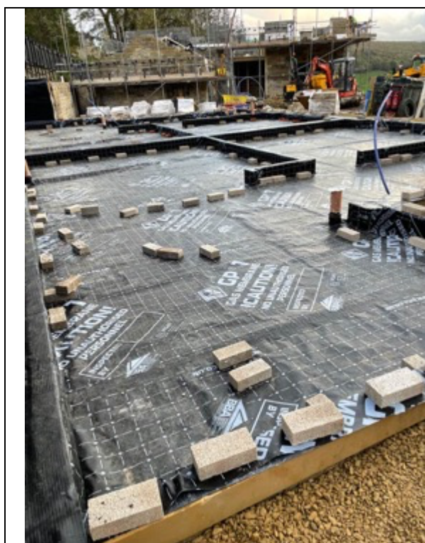
Plots 3 & 2 full line out installation
