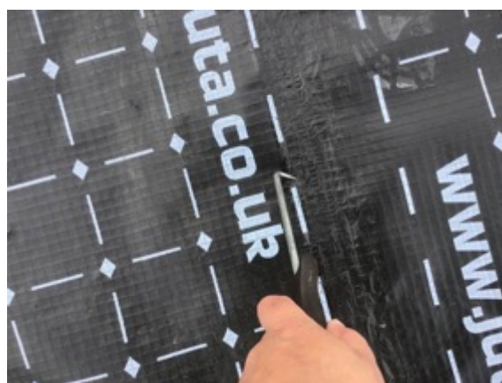
Hand welded joint being pick tested
