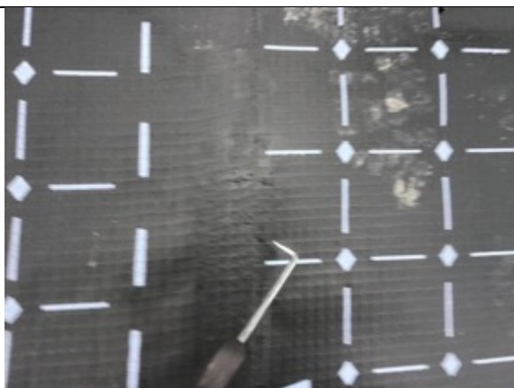
Plot 13 hand welded joint being pick tested
