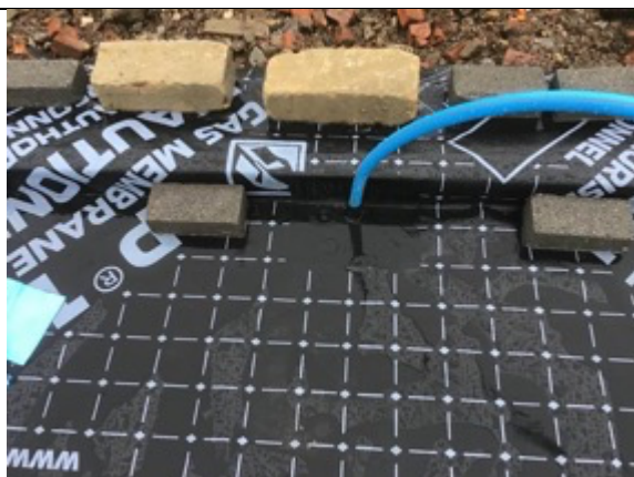
Plot 17 water pipe penetration sealed using SAGM
