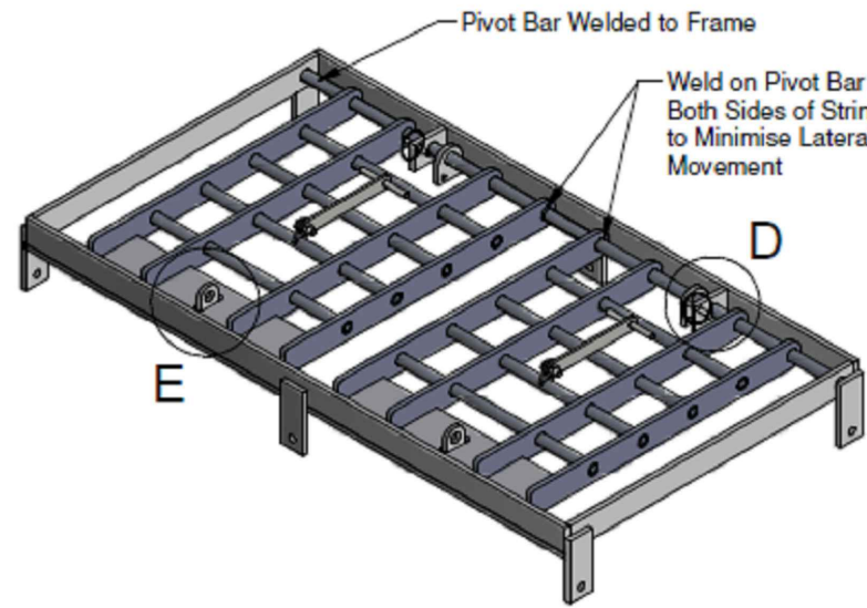
TYPICAL FALL ARREST GRILLE DETAIL (BY PETER SAVAGE LIMITED) (NTS)
