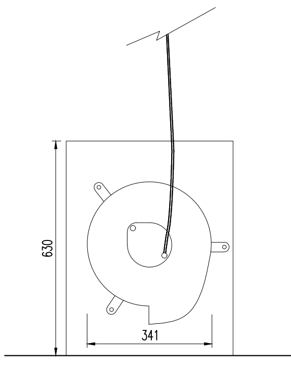
FLOW CONTROL FACE-ON VIEW (NTS)
