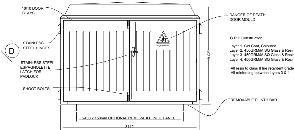
Elevation (B) (rear)
