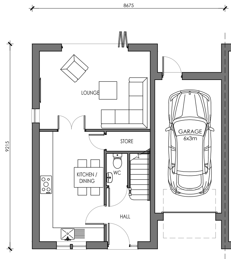
GROUND FLOOR
