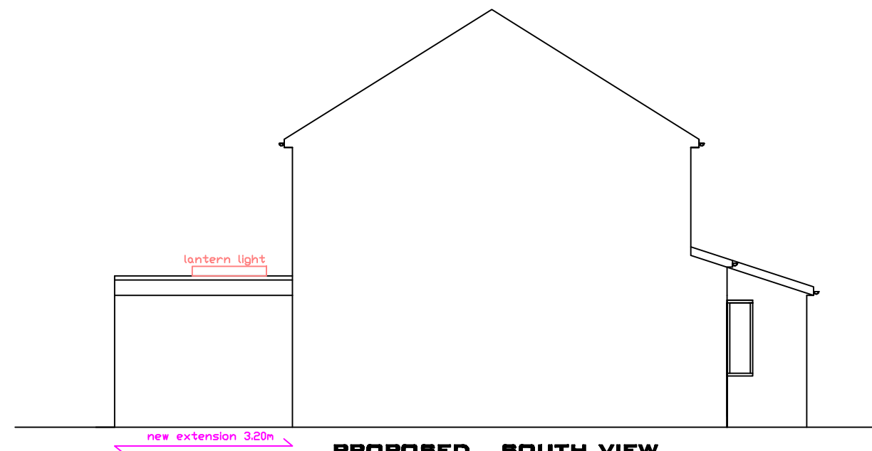
PROPOSED SOUTH VIEW 1:100
