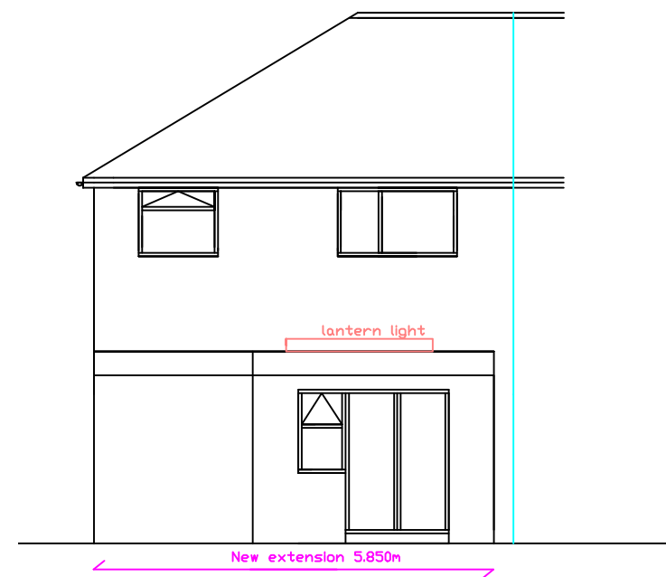
PROPOSED WEST VIEW 1:100
