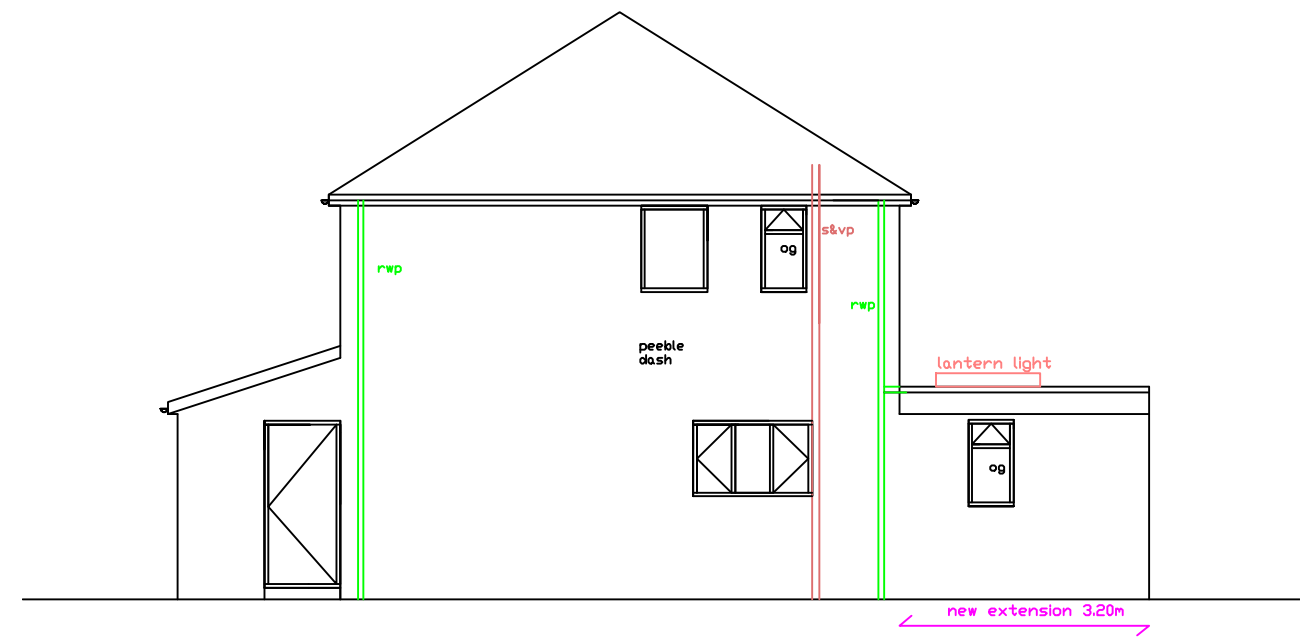
PROPOSED NORTH VIEW 1:100
