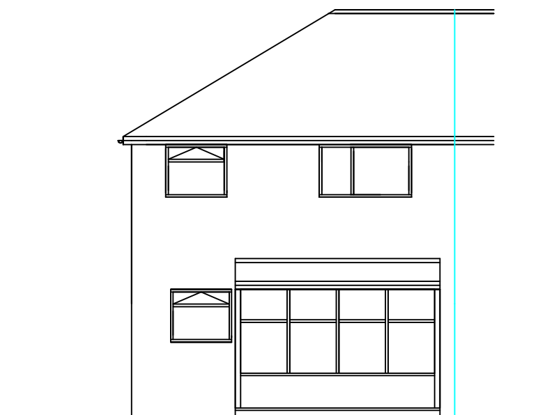
EXISTING WEST VIEW 1:100
