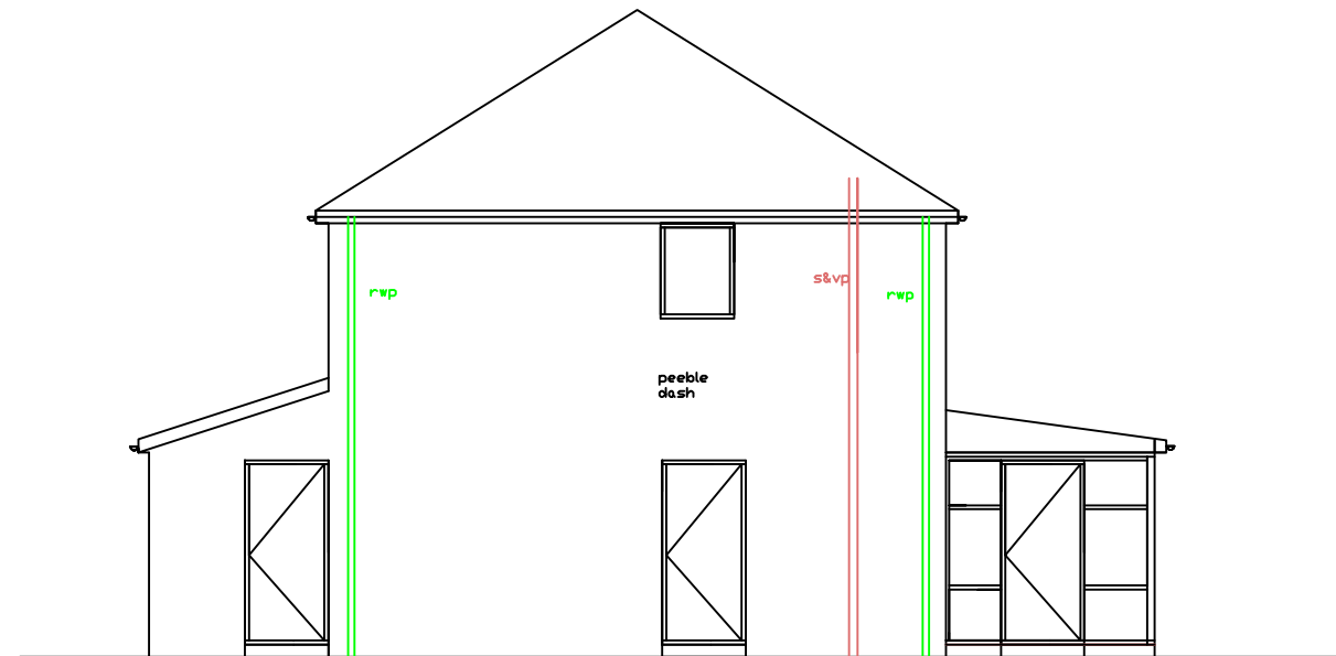
EXISTING NORTH VIEW 1:100
