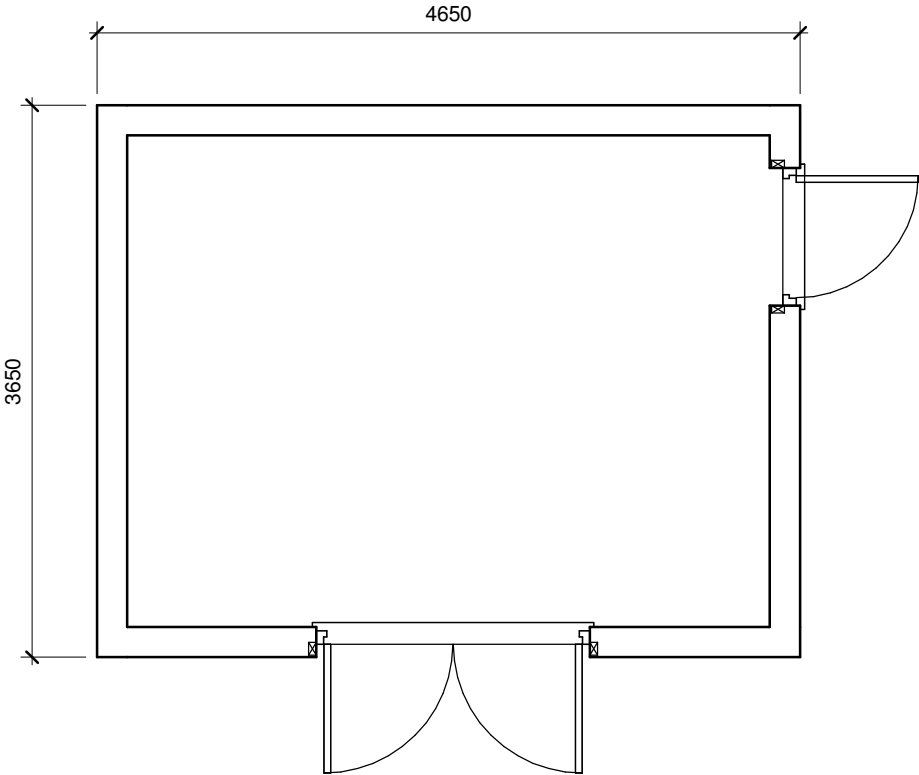
Ground Floor 1 : 50
