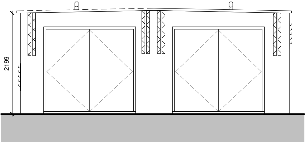
South 1 : 50
