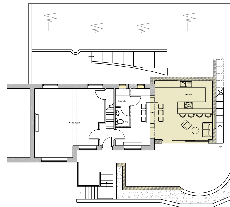
PROPOSED SITE PLAN 1:200
