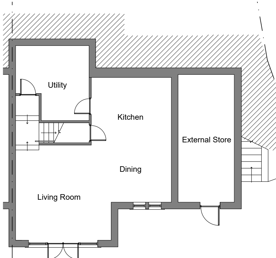
Basement - Existing
