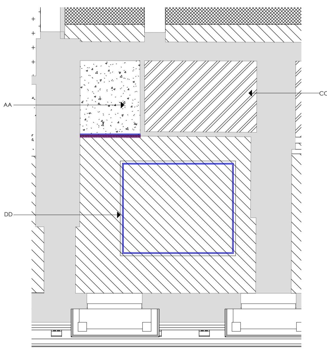
Reflected Ceiling Plan 1:50
