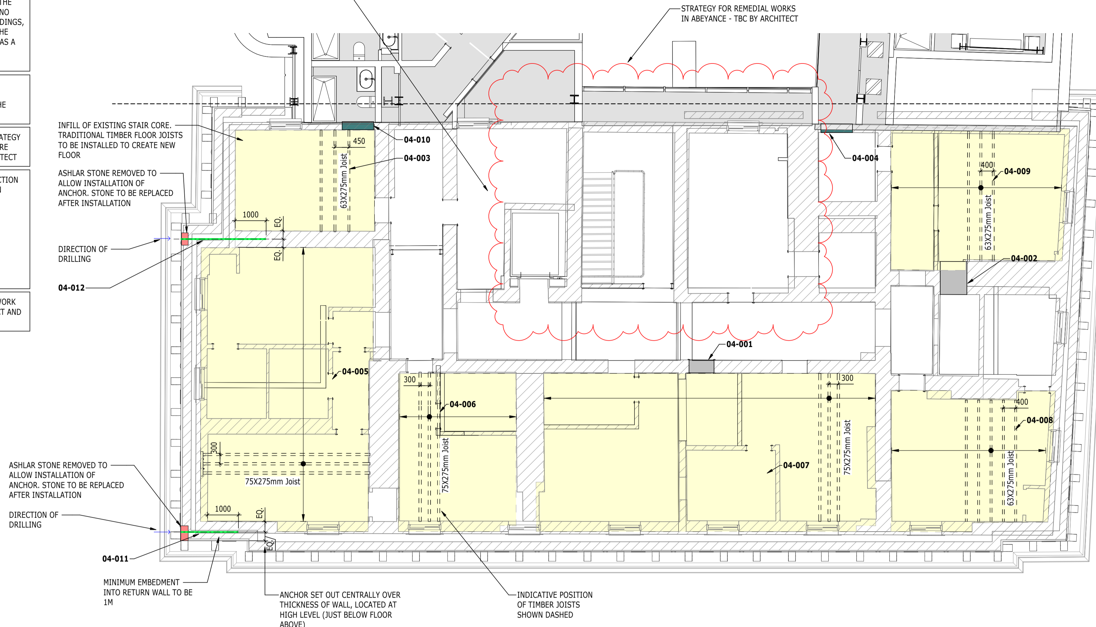
PLAN 1 : 75 BLOCK A - LEVEL 04
