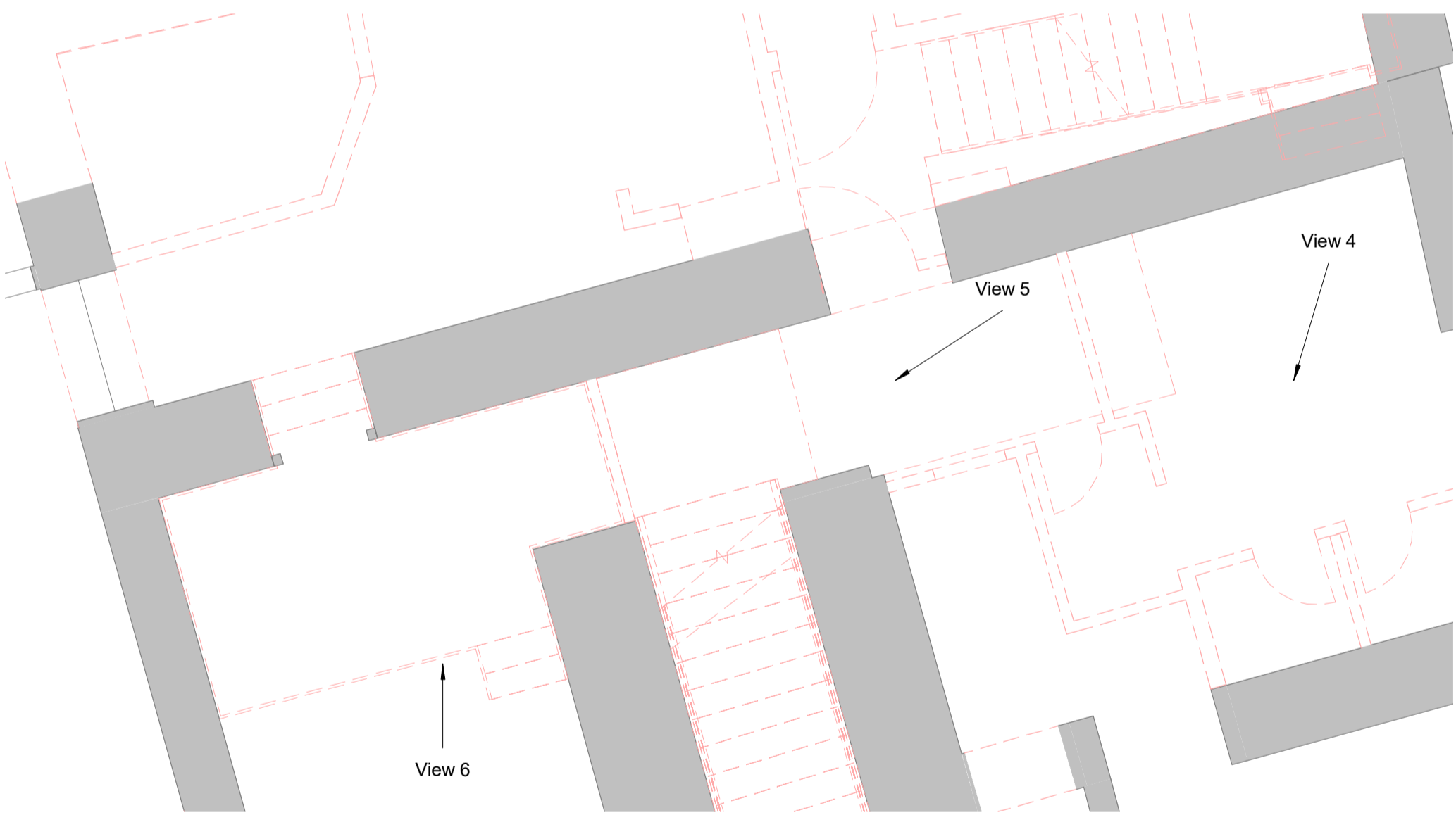
Block A Level -01 Layout Demolition - Callout 1 1 : 50
