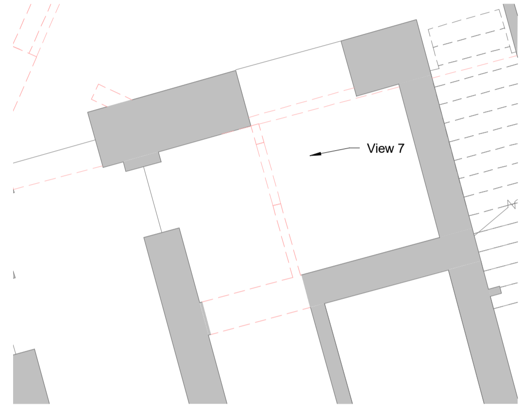
Block A Level -01 Layout Demolition - Callout 2 1 : 50
