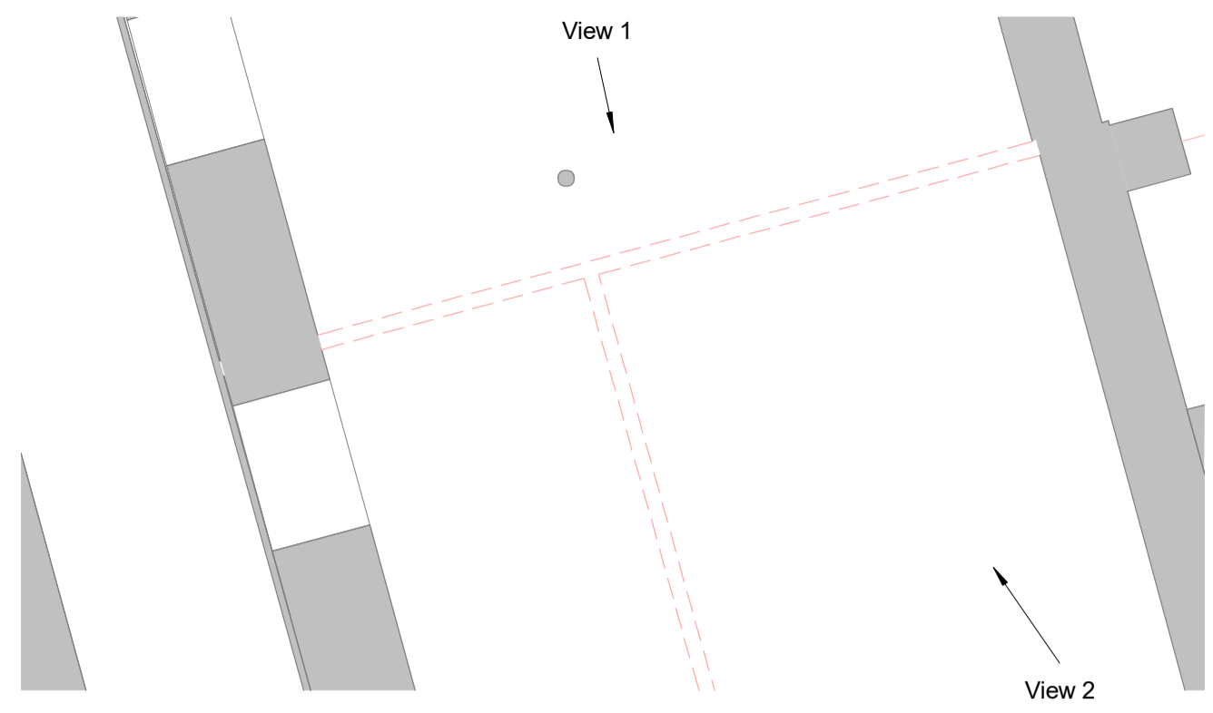
Block A Level -01 Layout Demolition - Callout 2 1 : 50
