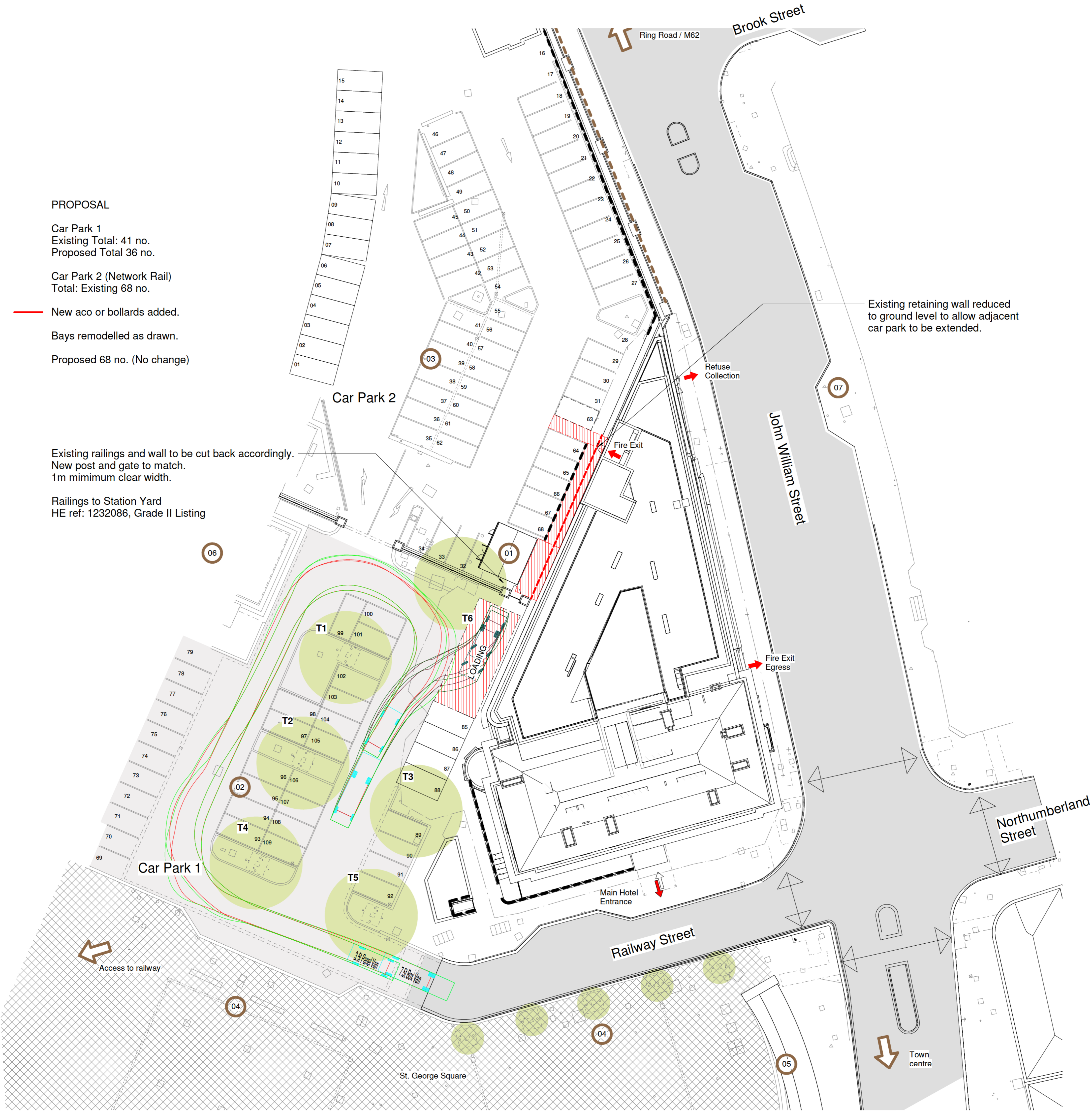
Vehicular Access Site Layout Option 1 1 : 200
