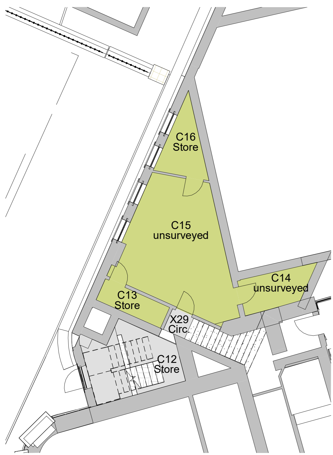
Block B Mezzanine Existing 1 : 100
