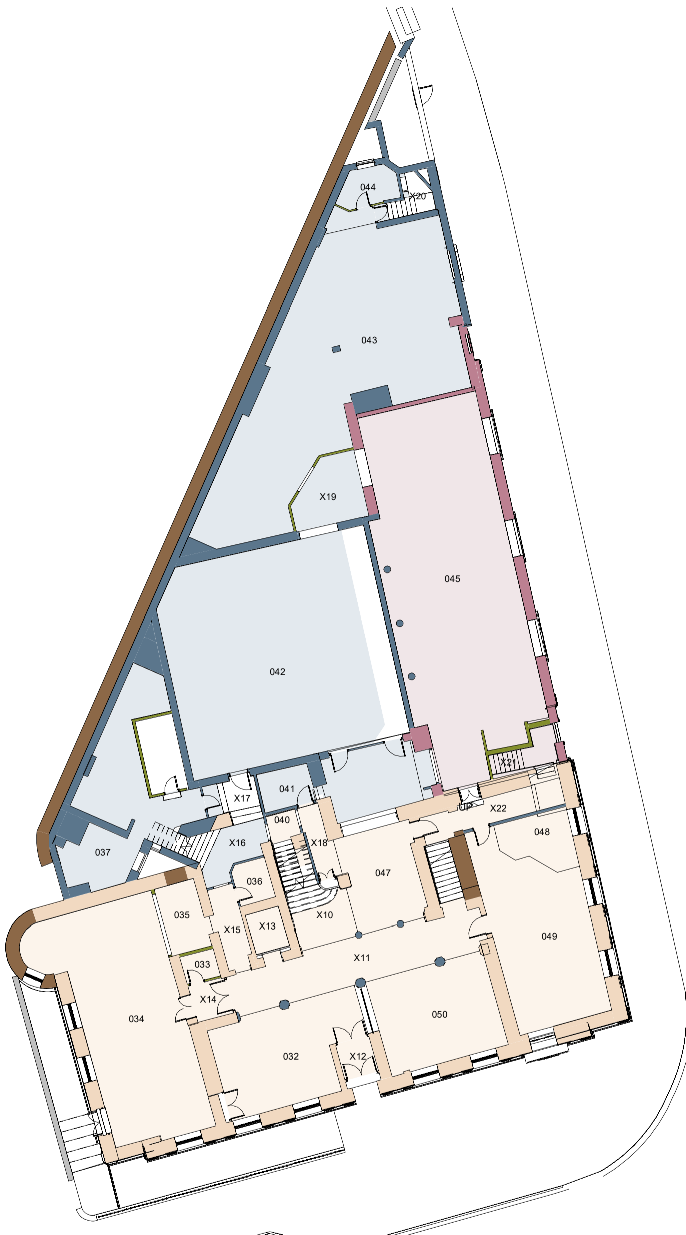
Phasing Plan - Level 00 1 : 200
