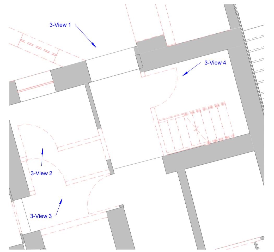
Demolition Plan - Level 03 - Callout 1 1 : 50
