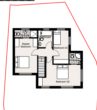
First Floor Plan As Proposed Scale 1:100
