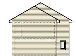
Side/ West Elevation As Proposed Scale 1:100
