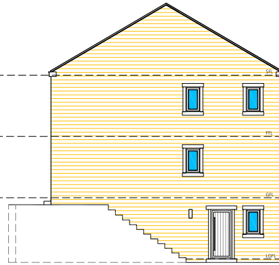
Proposed West Elevation Scale 1:100
