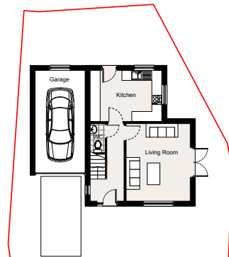
Ground Floor Plan As Proposed Scale 1:100
