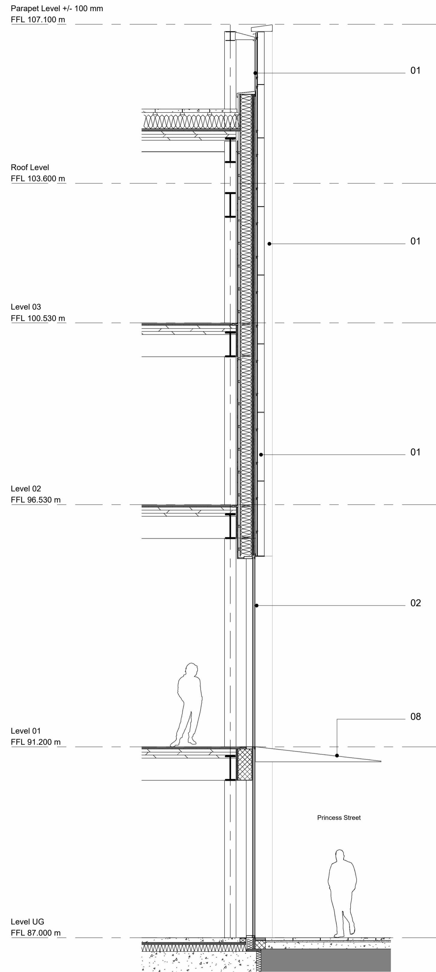
2 Bay Study Section - Ceramic and Curtain Wall Glazing 1 : 50
