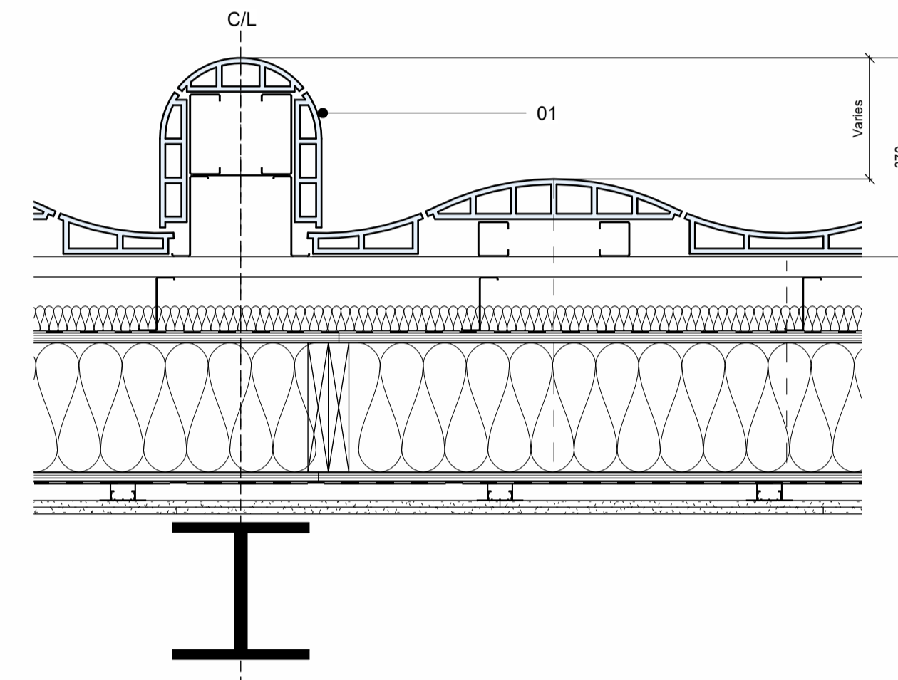
3 Solid Terracotta Wall Detail 1 : 10
