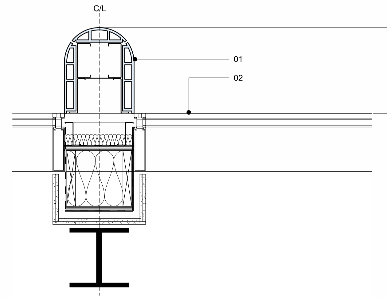
4 Terracotta and Curtain Wall Detail 1 : 10
