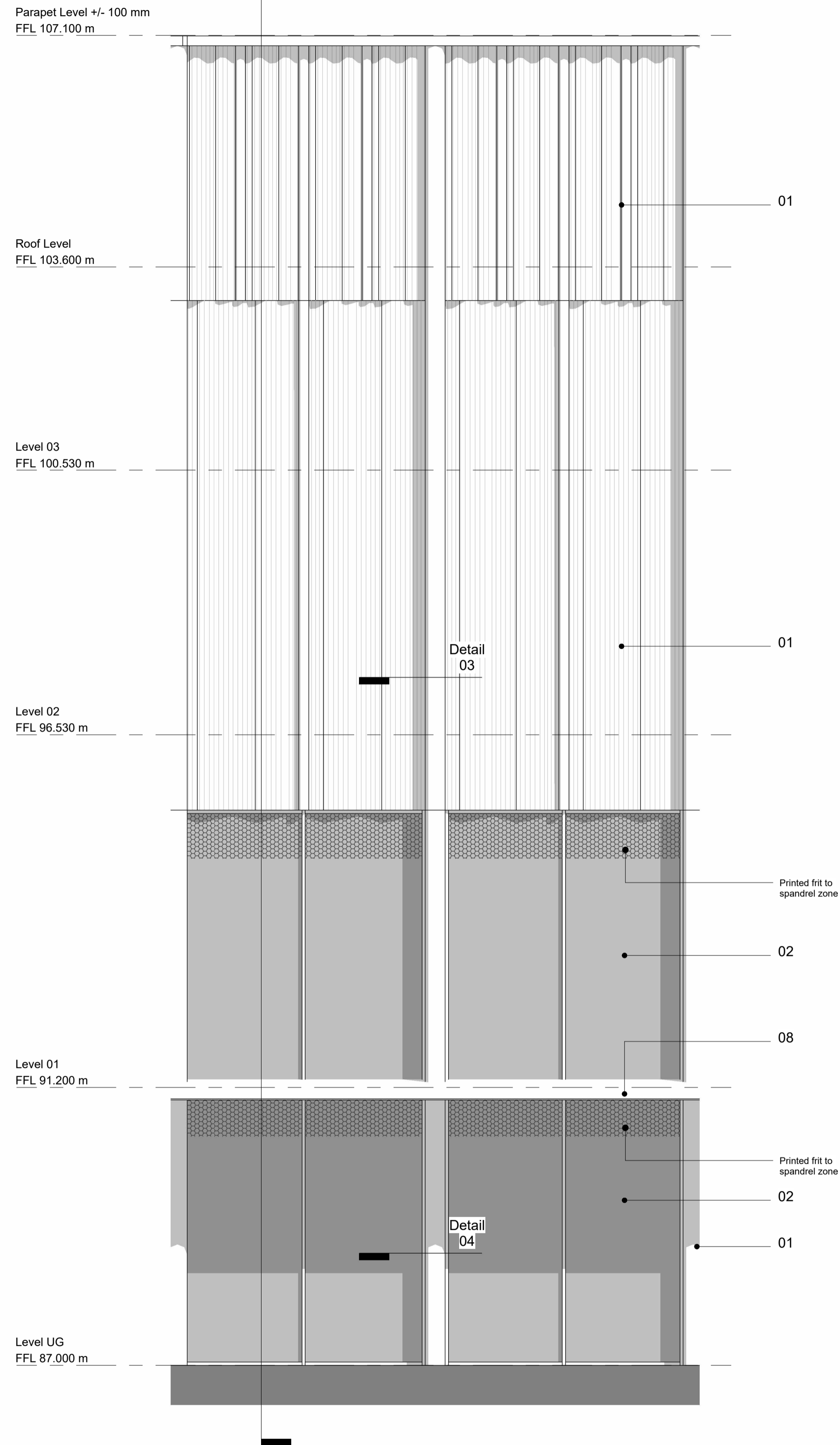
1 Bay Study Elevation - Ceramic and Curtain Wall Glazing 1 : 50
