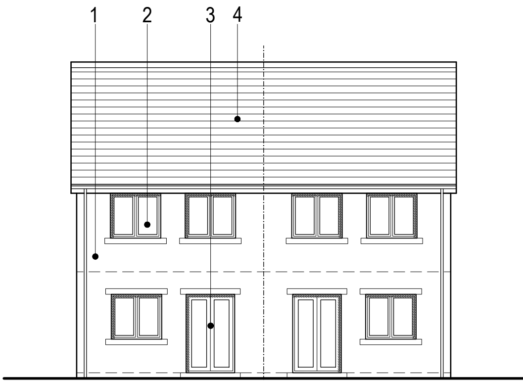
Rear Elevation
