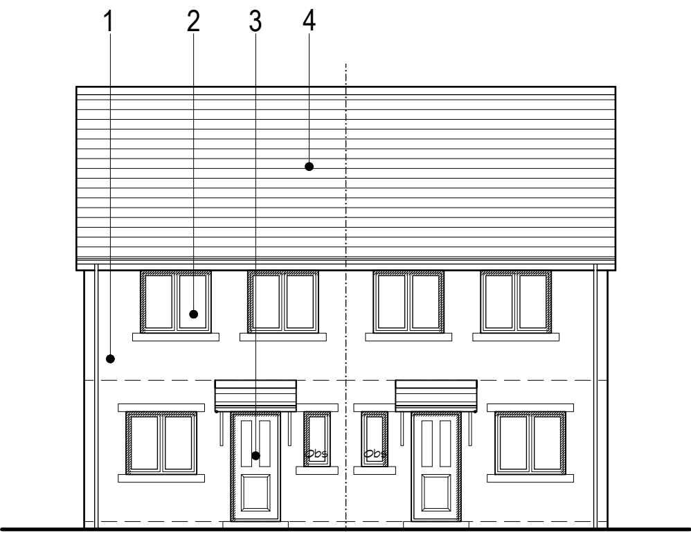
Front Elevation
