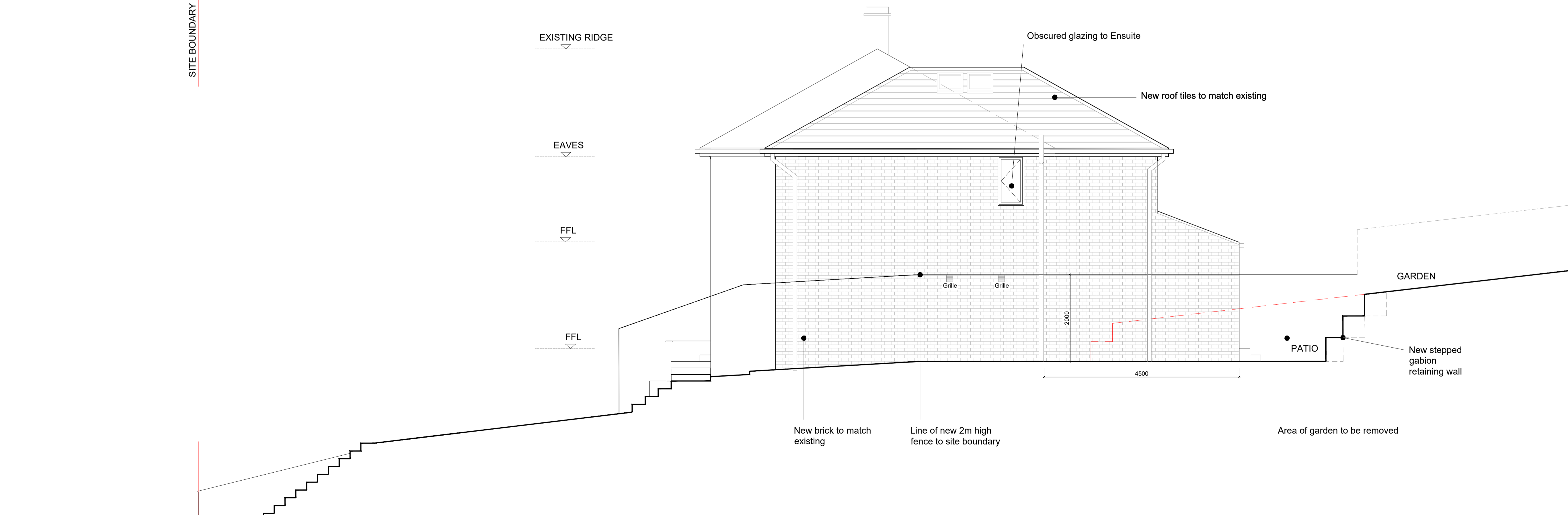
2 PROPOSED ELEVATION - SIDE 1:50@A1
