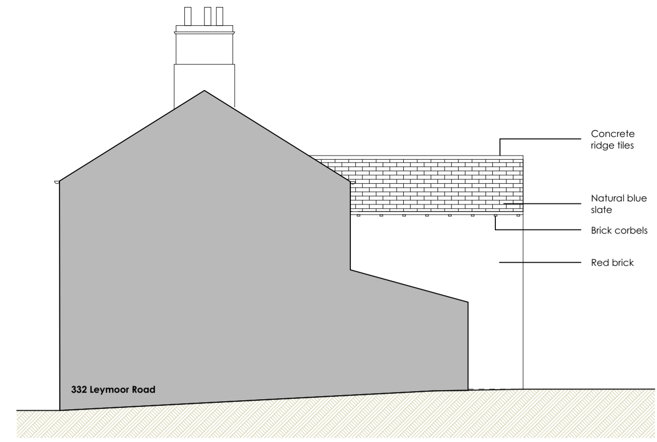
East Elevation
