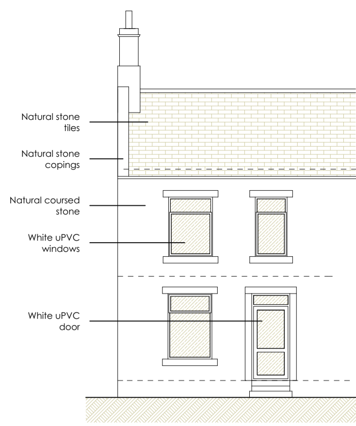
South Elevation
