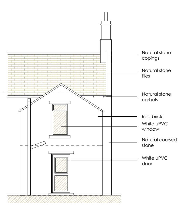
North Elevation
