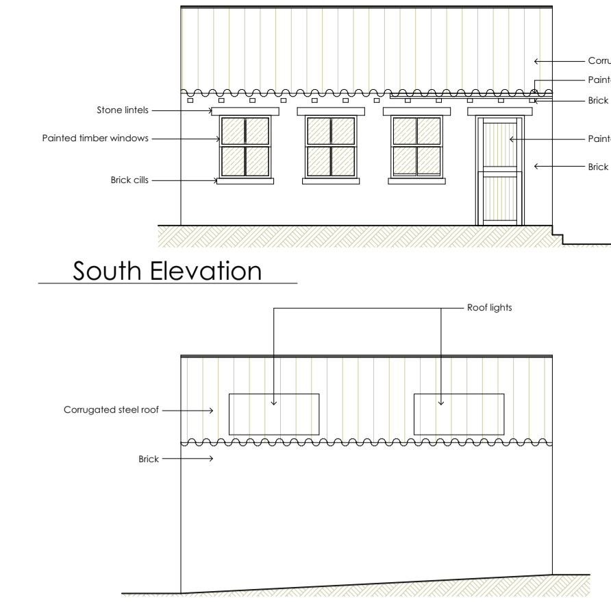
South Elevation
