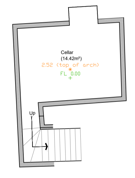
Basement Floor
