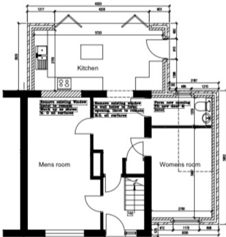
Ground Floor Layout as Proposed
