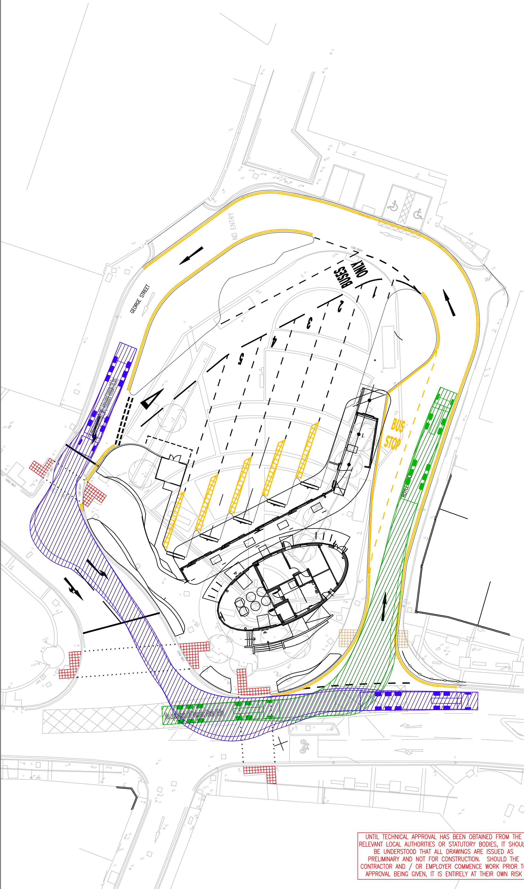
16.5m ARTICULATED HGV LEFT IN TO BUS STATION FROM WESTGATE & EXITING LEFT ONTO WESTGATE
