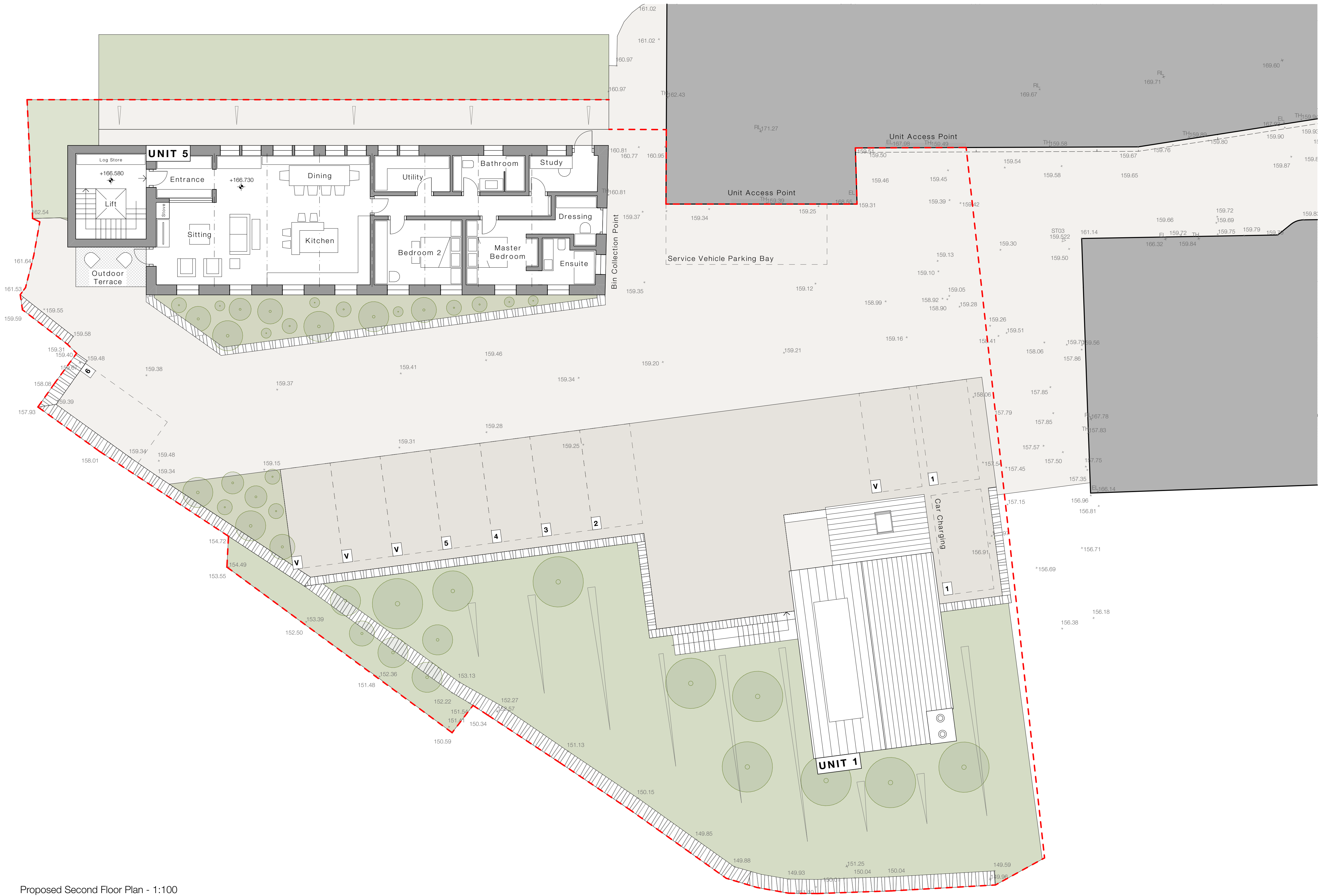
Proposed Second Floor Plan - 1:100
