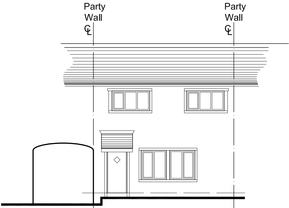
EXISTING SOUTH EAST (REAR) ELEVATION
