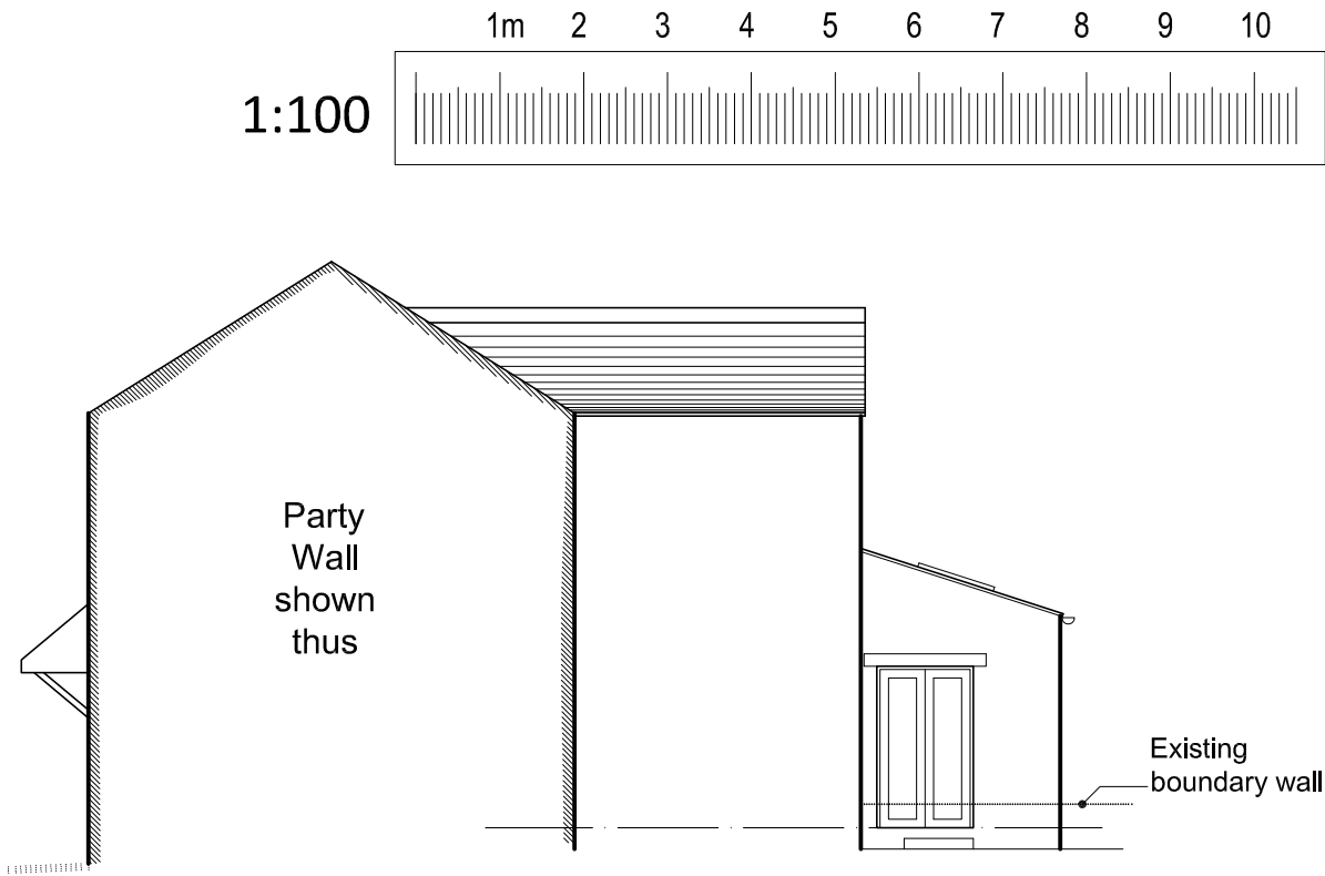
EXISTING SOUTH EAST (SIDE) ELEVATION
