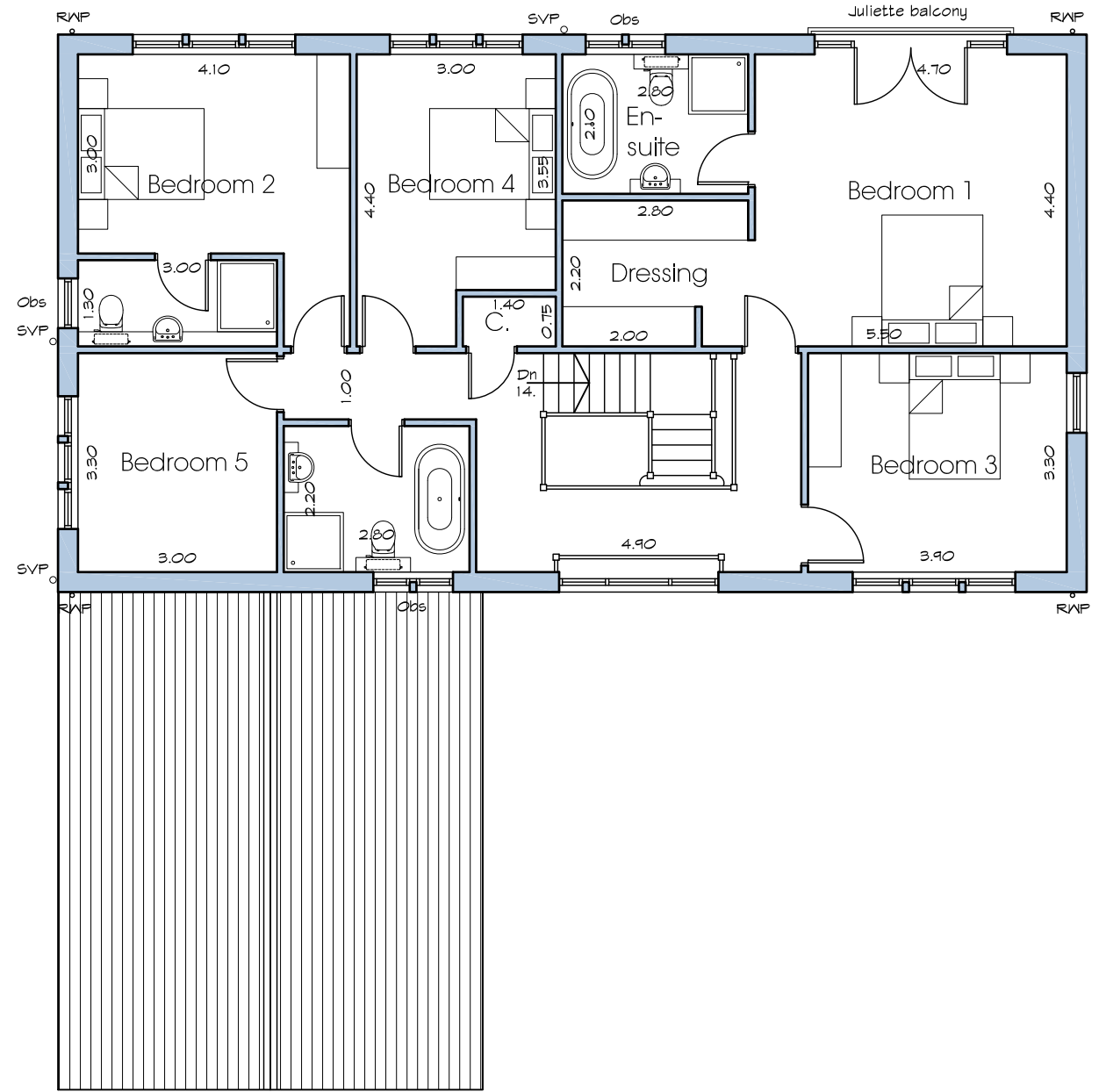
2 First Floor GA Plan 1 : 100
