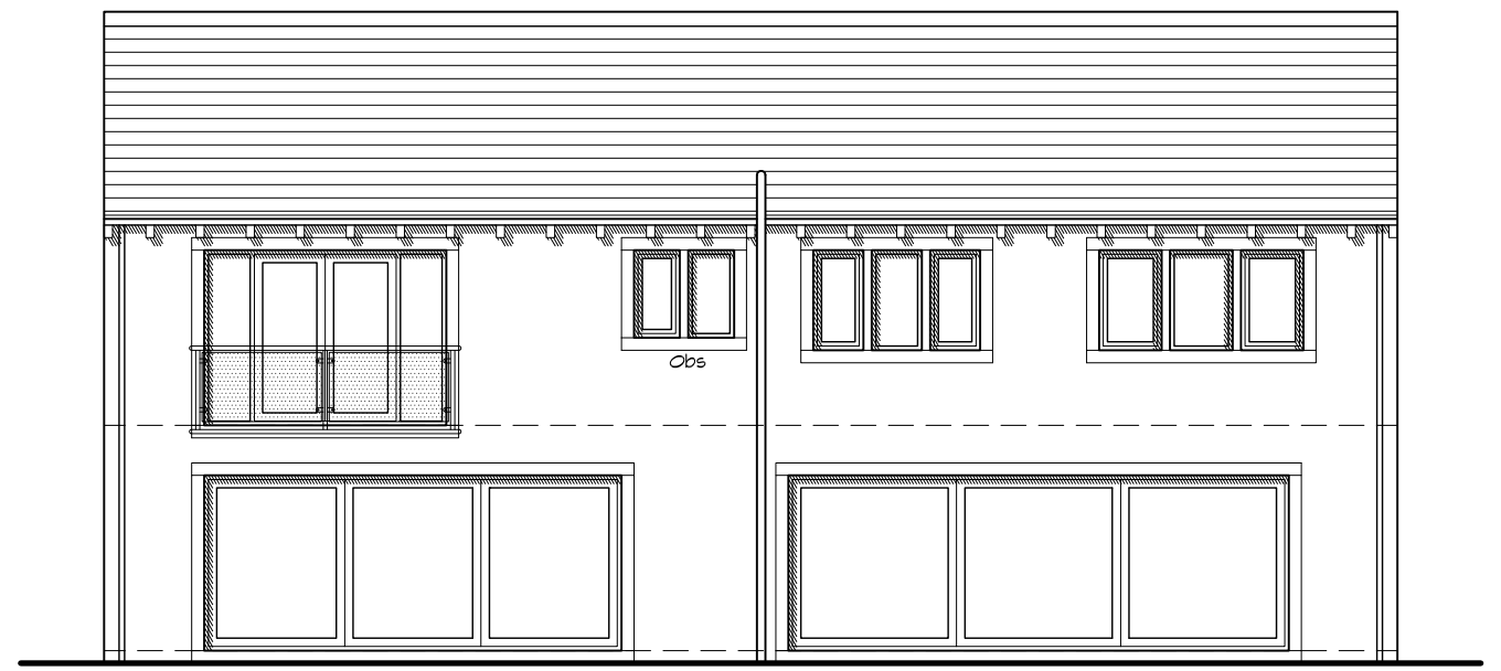
4 Rear Elevation 1 : 100
