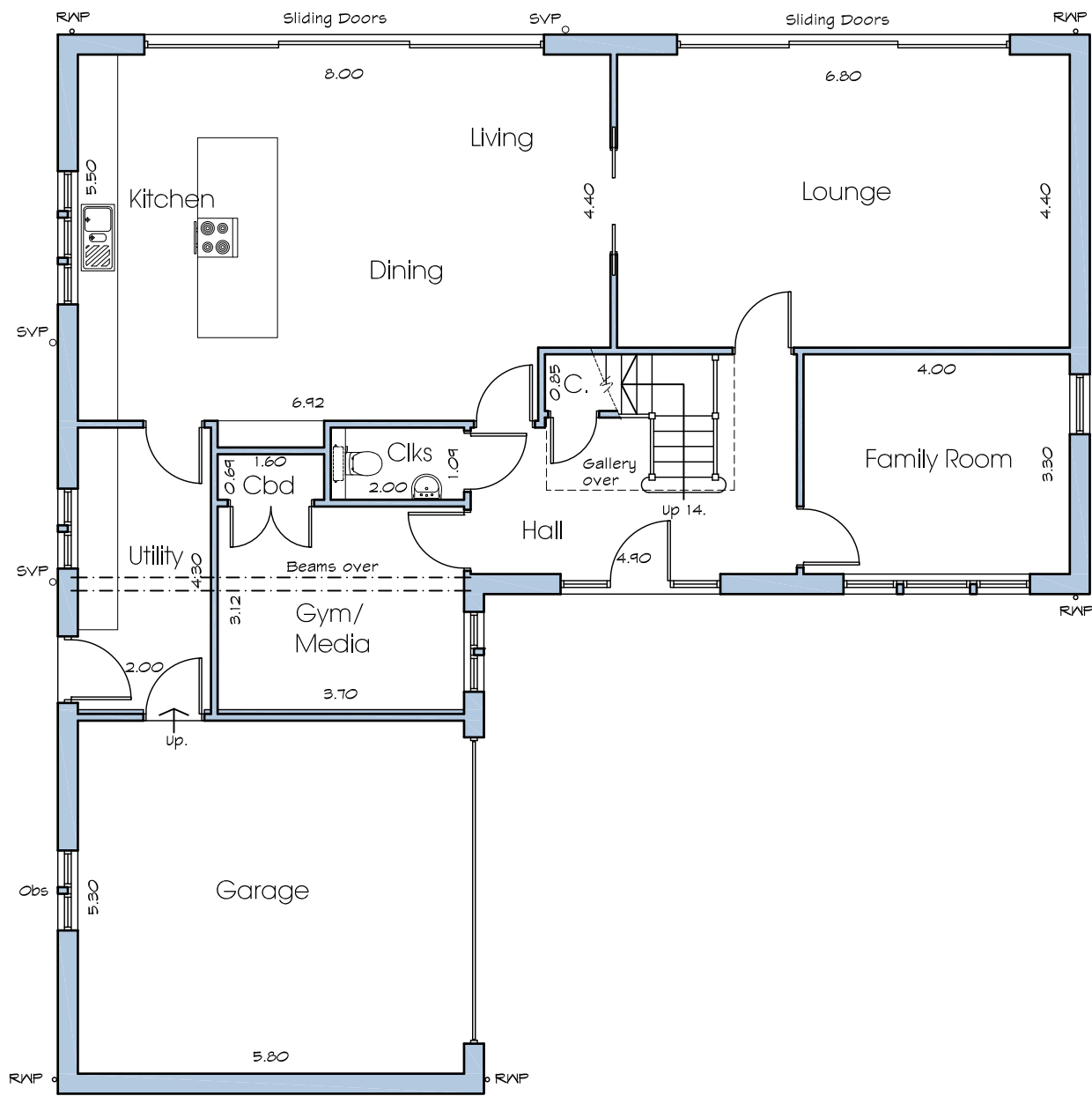
1 Ground Floor GA Plan 1 : 100
