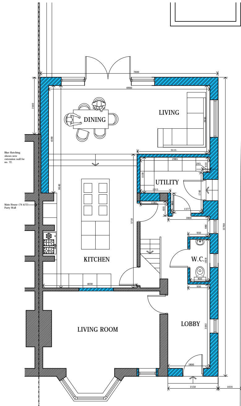
1. Proposed Ground Floor Plan Scale 1:100
