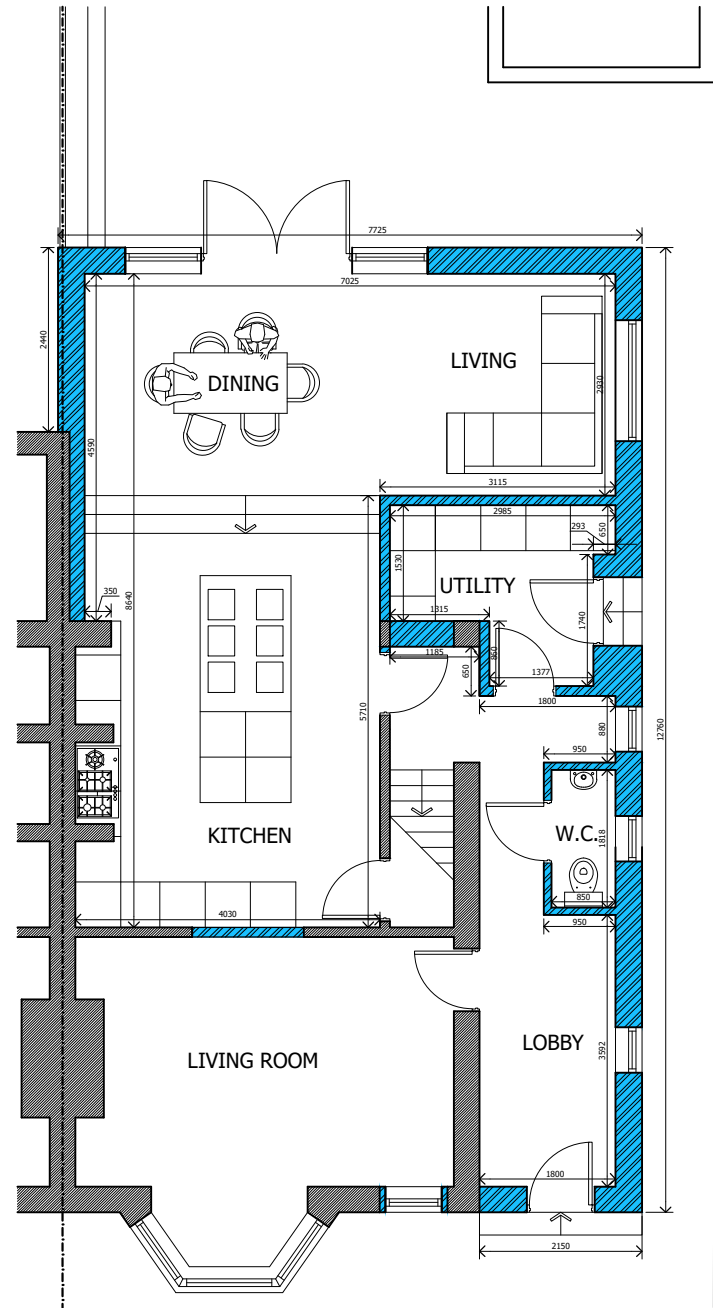
1. Proposed Ground Floor Plan Scale 1:100
