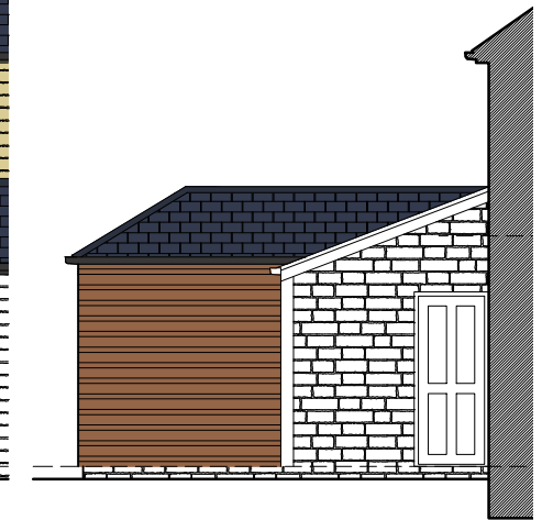
4. Existing West Elevation Scale 1:100
