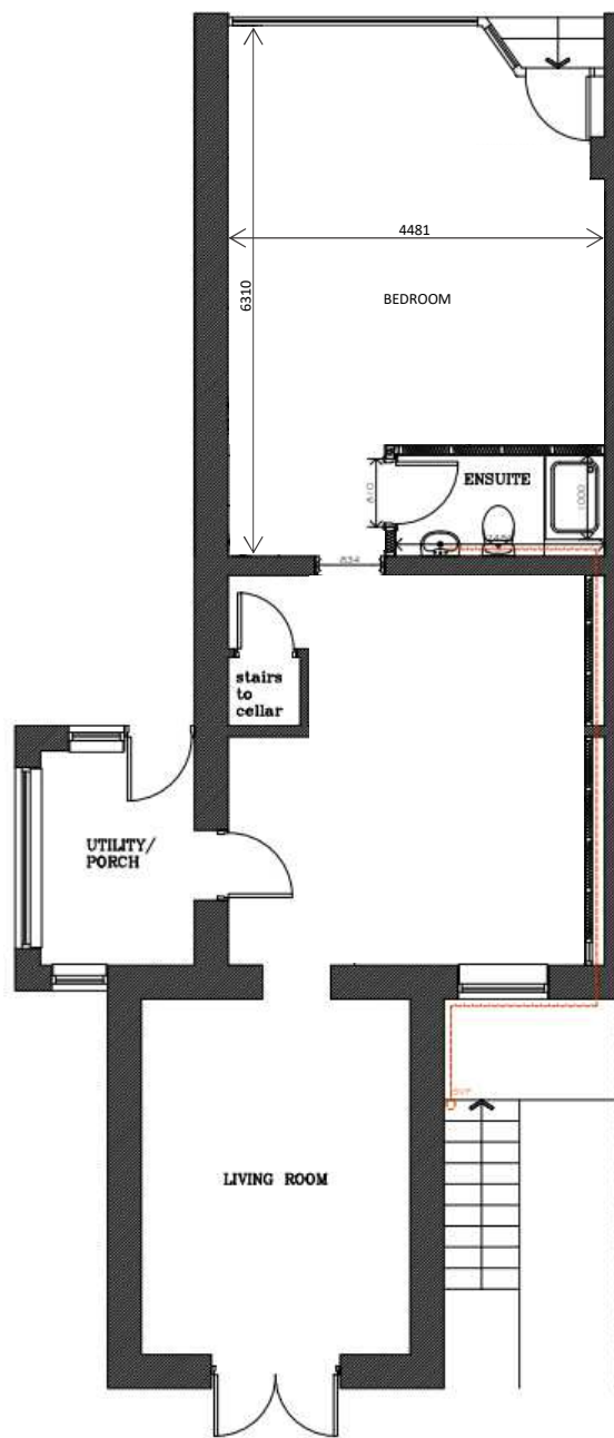
EXISTING GROUND FLOOR LAYOUT 1: 50
