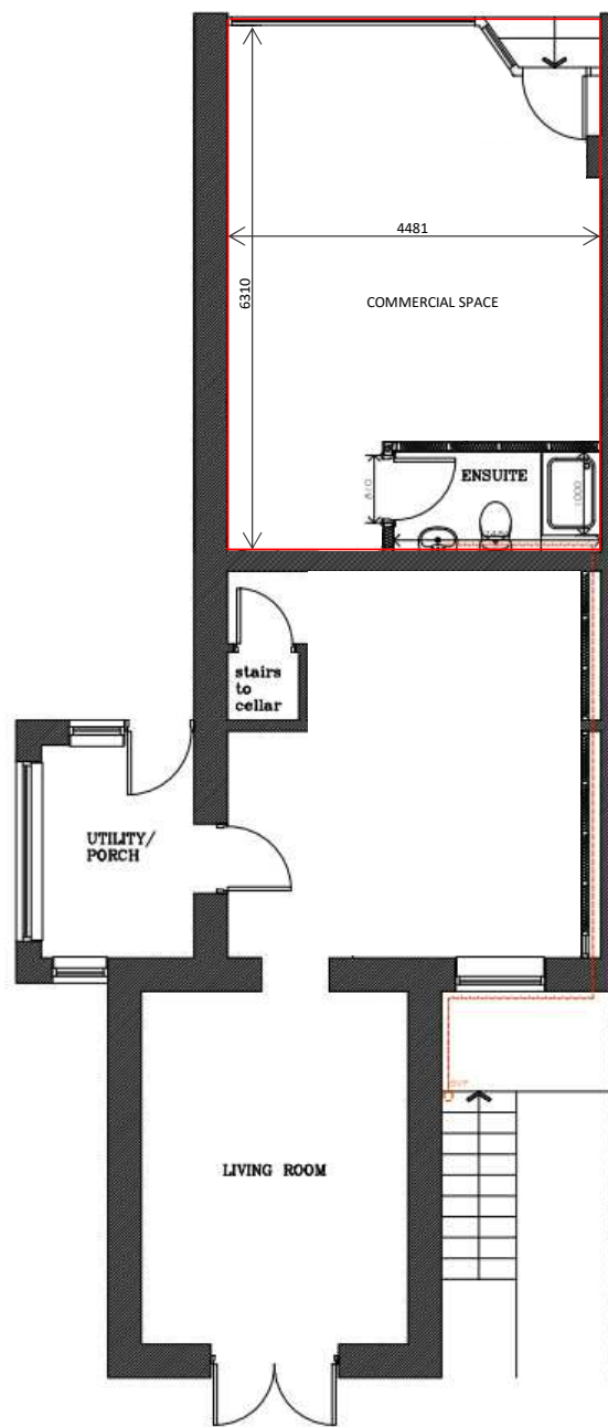
PROPOSED GROUND FLOOR LAYOUT 1: 50
