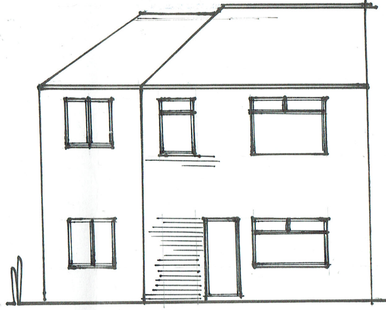
PROPOSED FRONT
