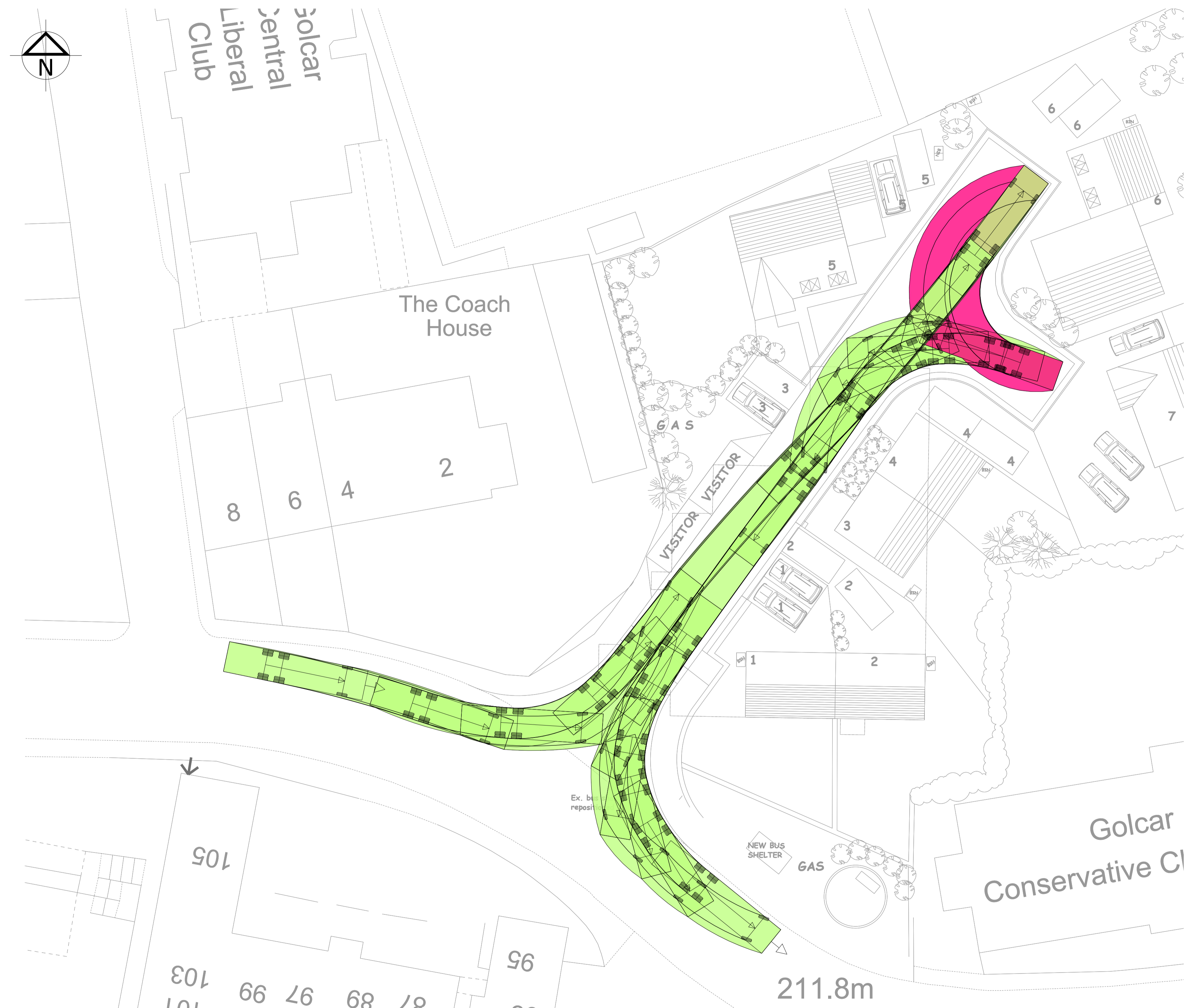
Refuse Vehicle - Tracking Plan 1 Scale 1:200
