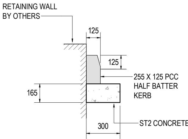
HALF BATTER KERB DETAIL RET WALL (HBRW)
