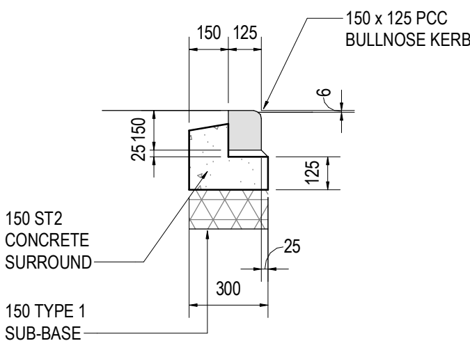
BULL NOSE KERB DETAIL (BN)
