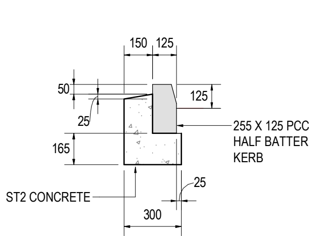
HALF BATTER KERB DETAIL (HB)
