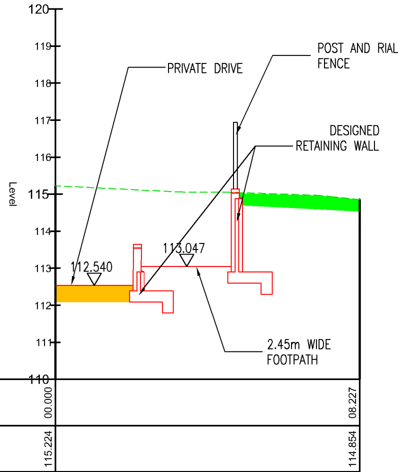
PROPOSED PROW SECTION A-A SCALE: H 1:100, V 1:100
