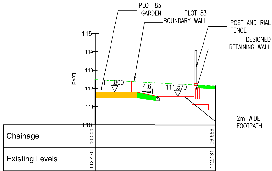
PROPOSED PROW SECTION B-B SCALE: H 1:100, V 1:100
