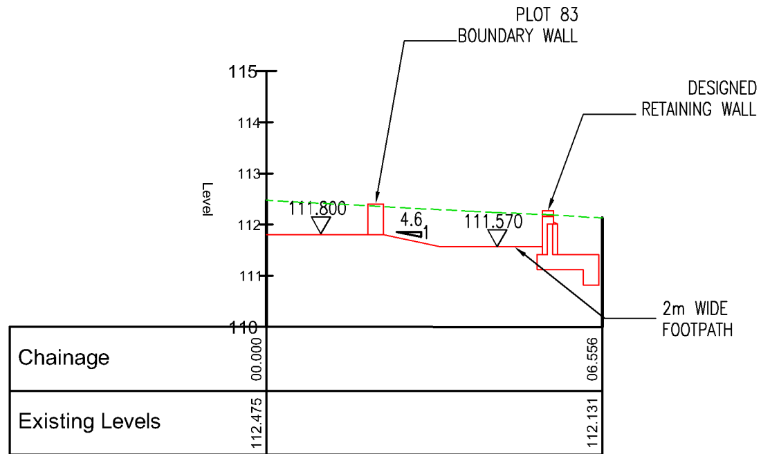
PROPOSED PROW SECTION B-B SCALE: H 1:100, V 1:100
