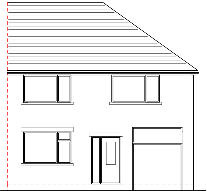
front (south east) elevation
