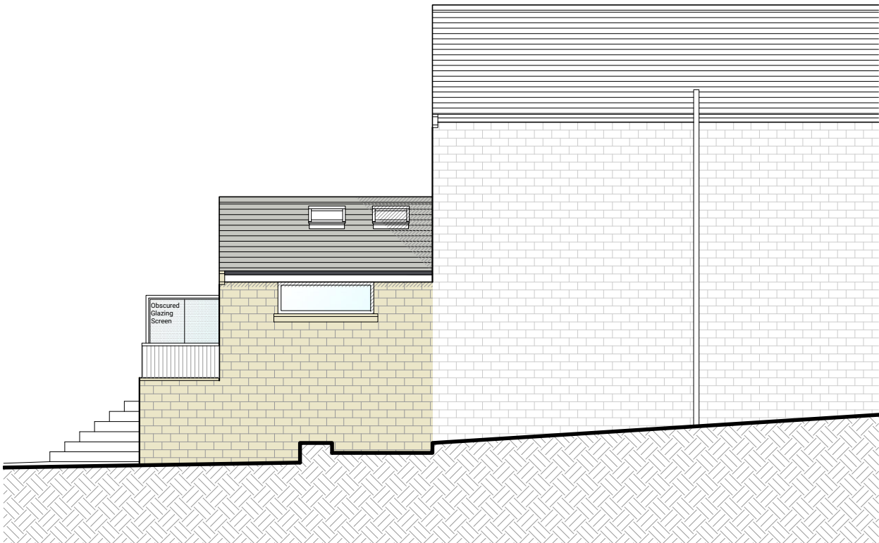
W Side Elevation Scale 1:100
