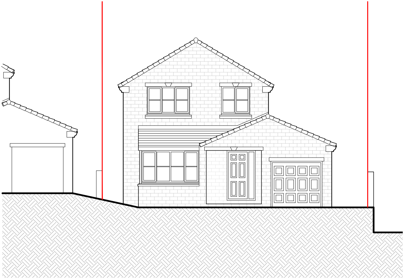
S Front Elevation Scale 1:100
