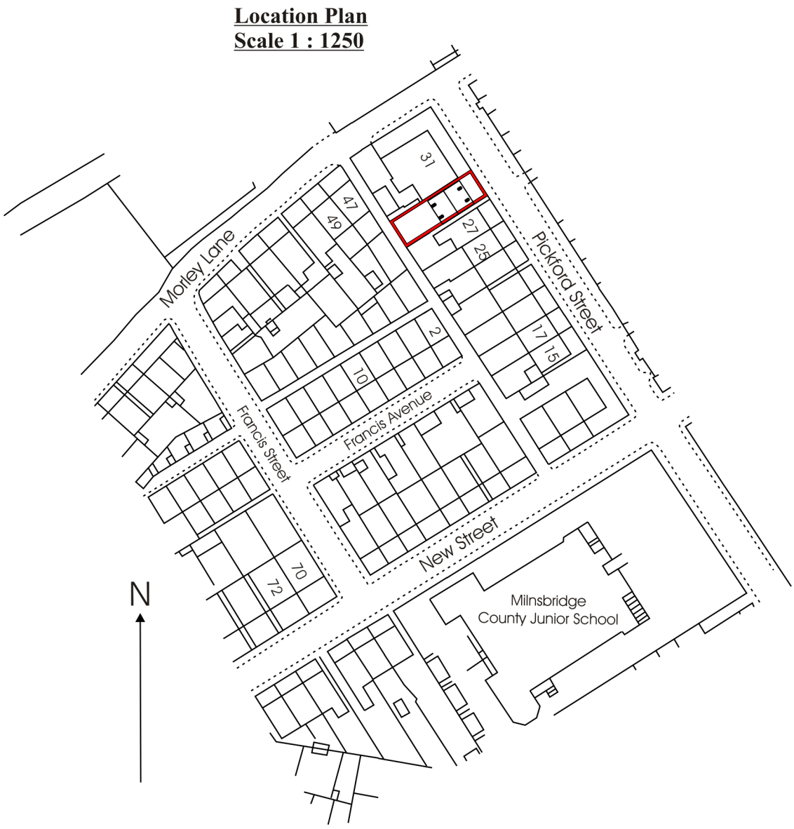
1 Location Plan 1 : 1250
