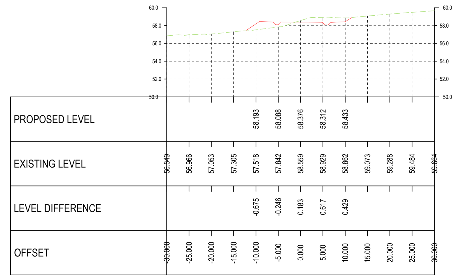
Road 3 Alignment CH 0+060.00 SCALES: H 1:500, V 1:250
