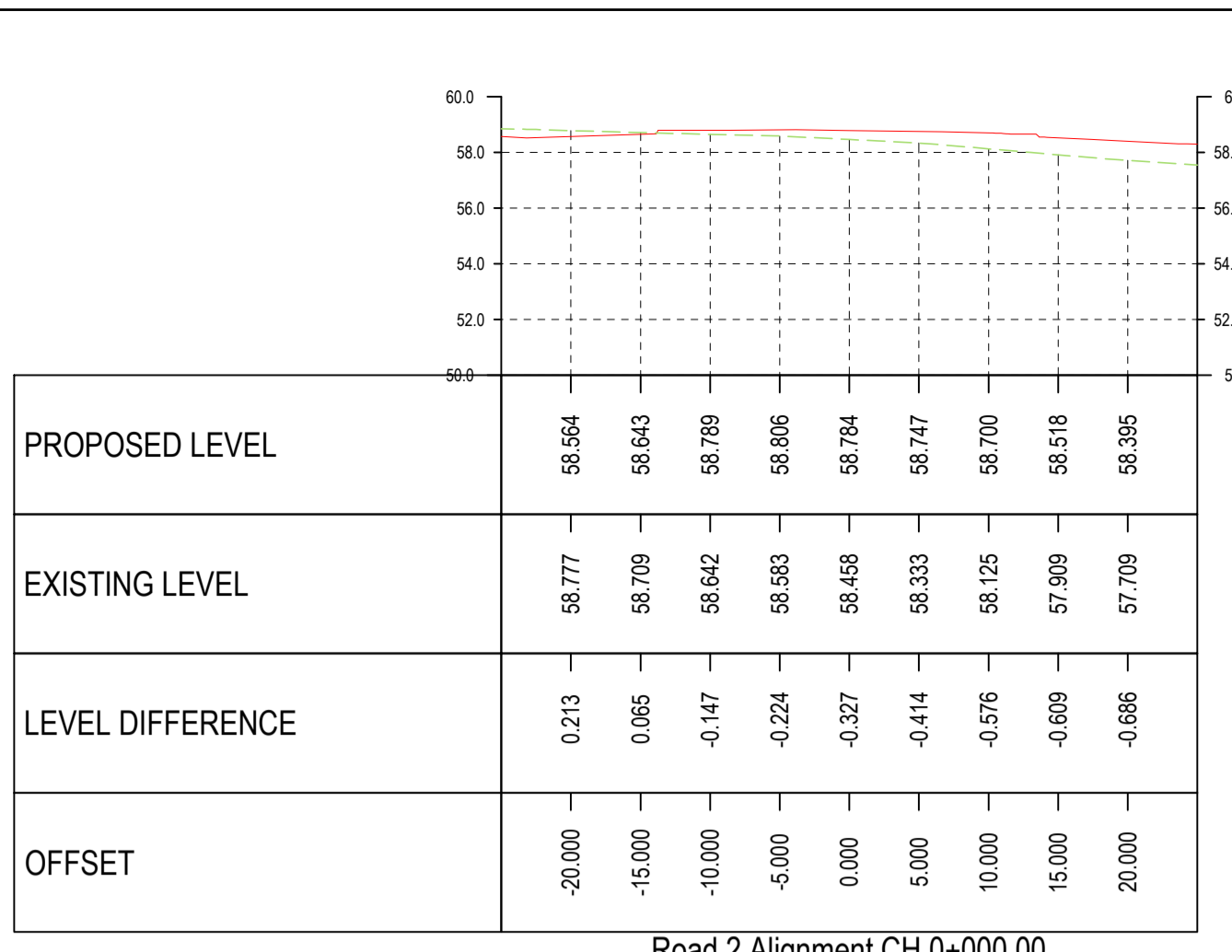
Road 2 Alignment CH 0+000.00 SCALES: H 1:500, V 1:250
