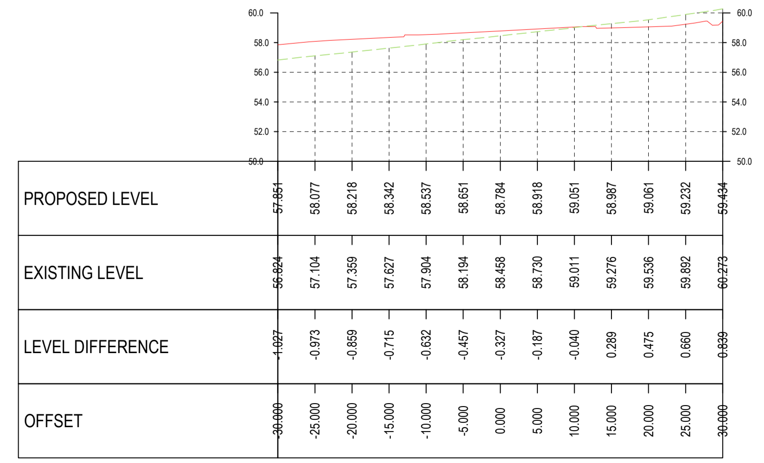
Road 3 Alignment CH 0+000.00 SCALES: H 1:500, V 1:250
