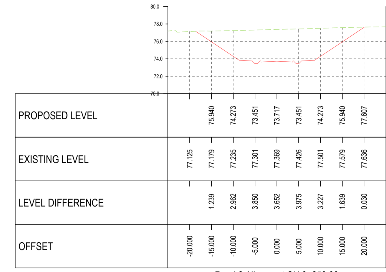
Road 2 Alignment CH 0+250.00 SCALES: H 1:500, V 1:250
