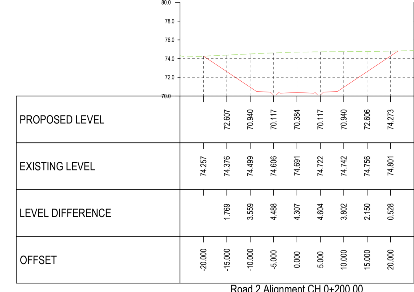
Road 2 Alignment CH 0+200.00 SCALES: H 1:500, V 1:250
