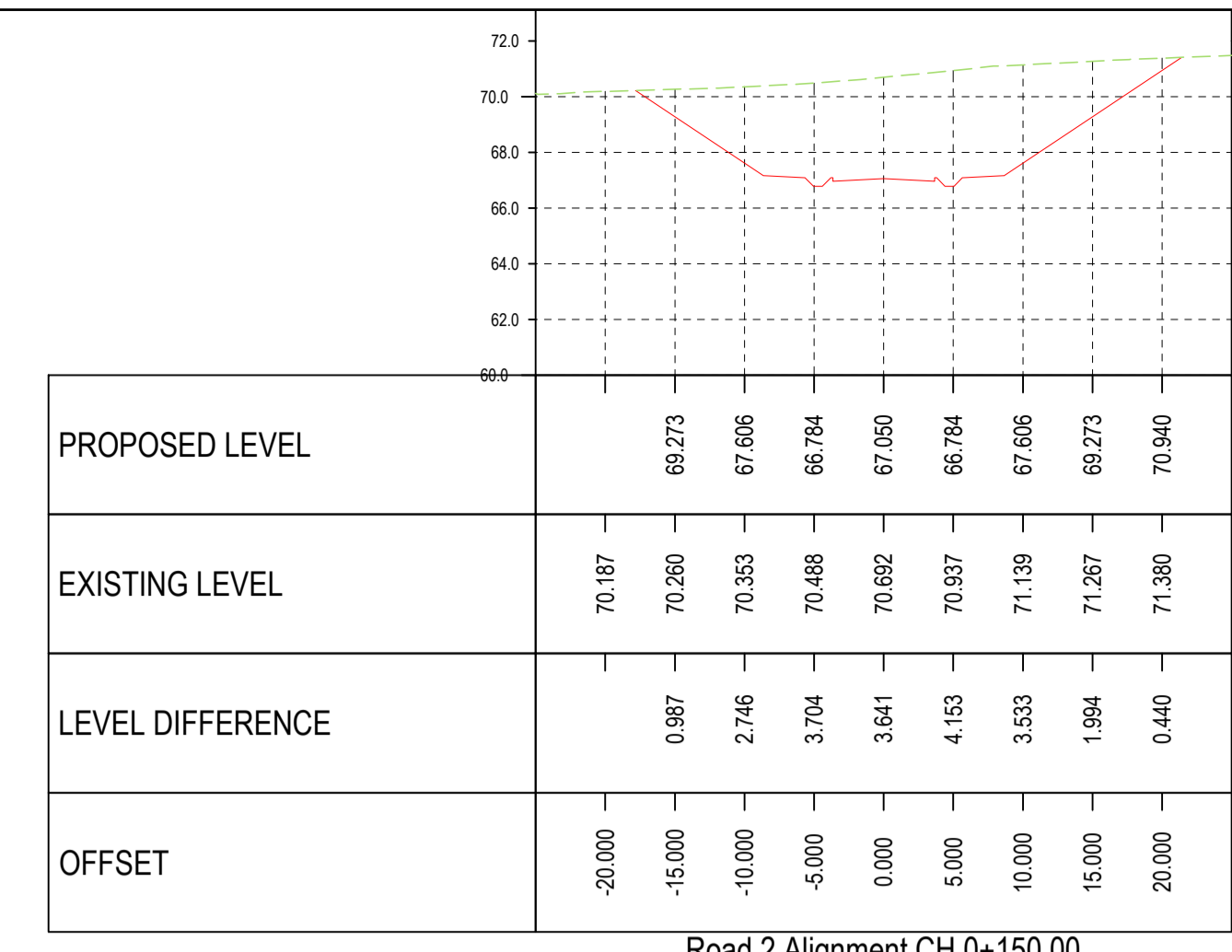
Road 2 Alignment CH 0+150.00 SCALES: H 1:500, V 1:250
