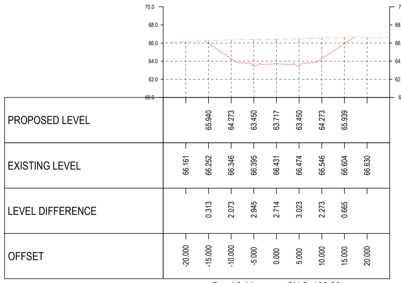
Road 2 Alignment CH 0+100.00 SCALES: H 1:500, V 1:250
