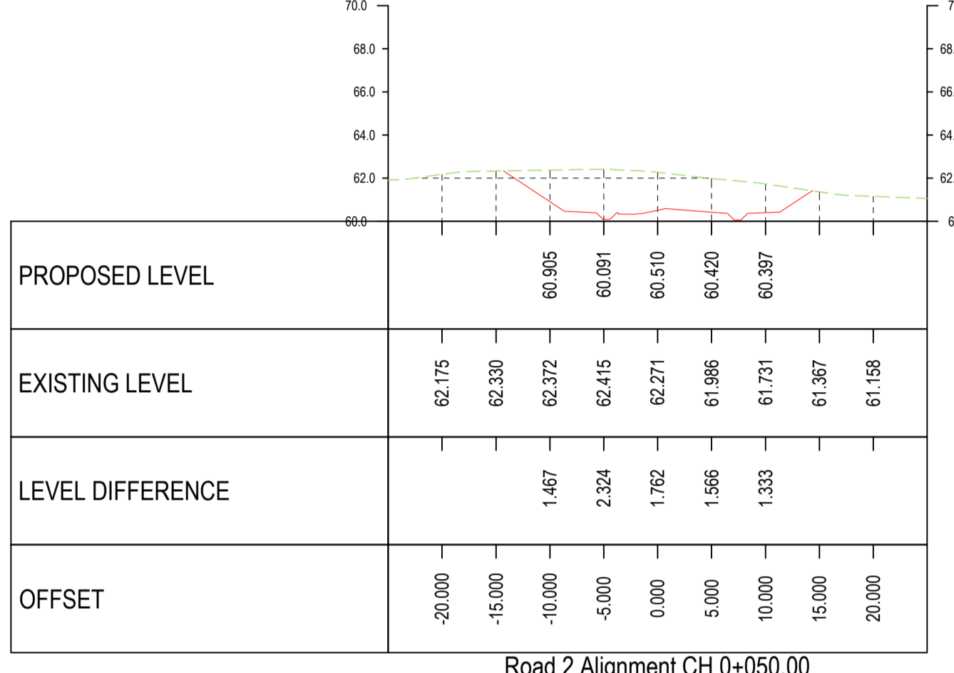
Road 2 Alignment CH 0+050.00 SCALES: H 1:500, V 1:250
