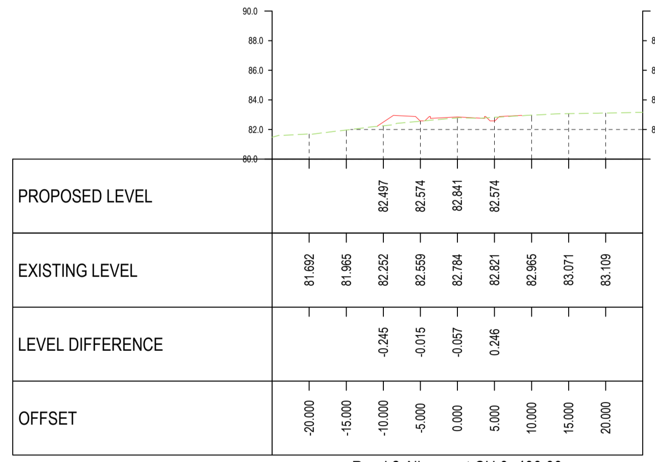
Road 2 Alignment CH 0+400.00 SCALES: H 1:500, V 1:250
