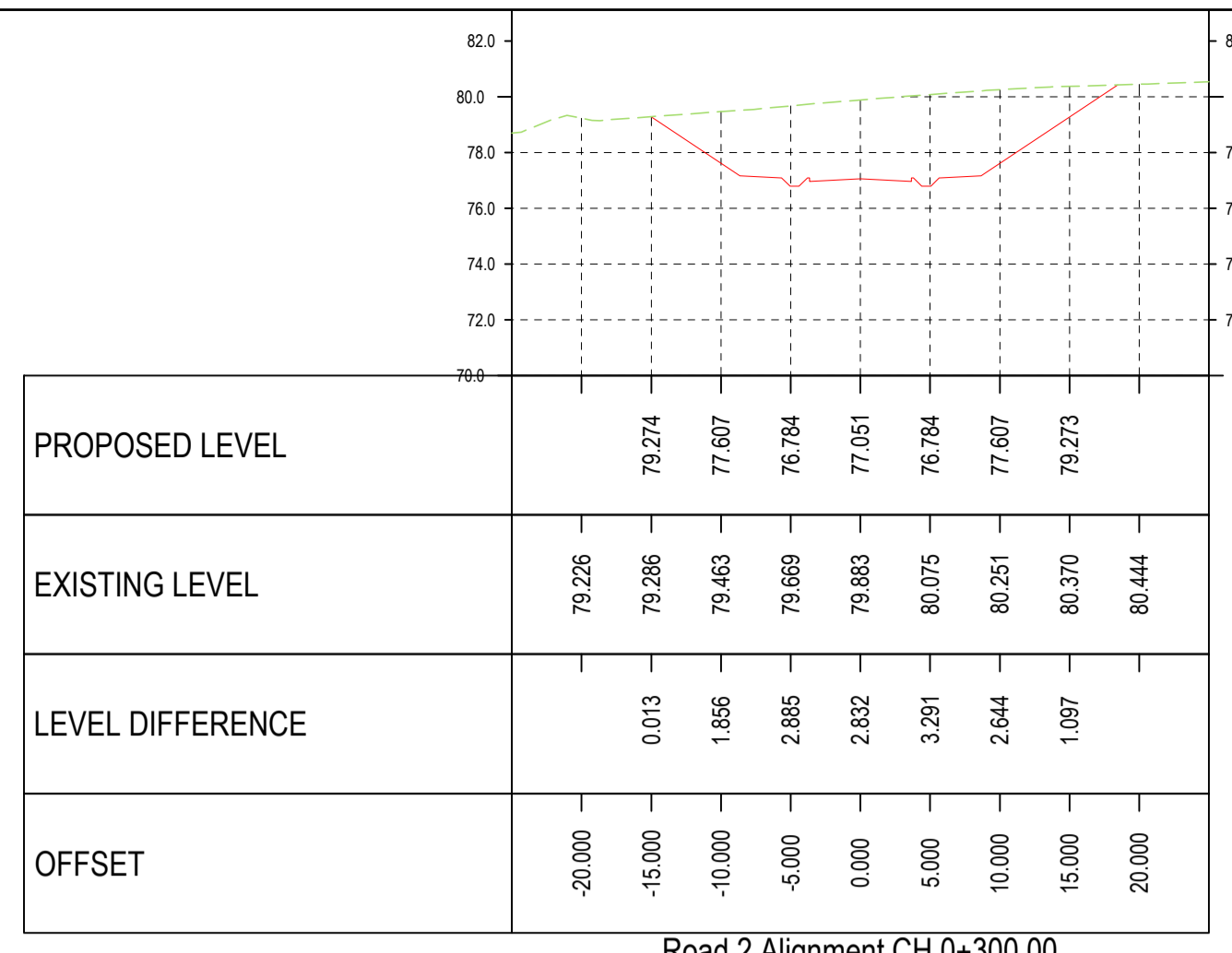
Road 2 Alignment CH 0+300.00 SCALES: H 1:500, V 1:250
