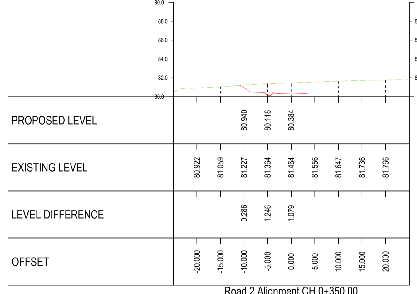
Road 2 Alignment CH 0+350.00 SCALES: H 1:500, V 1:250
